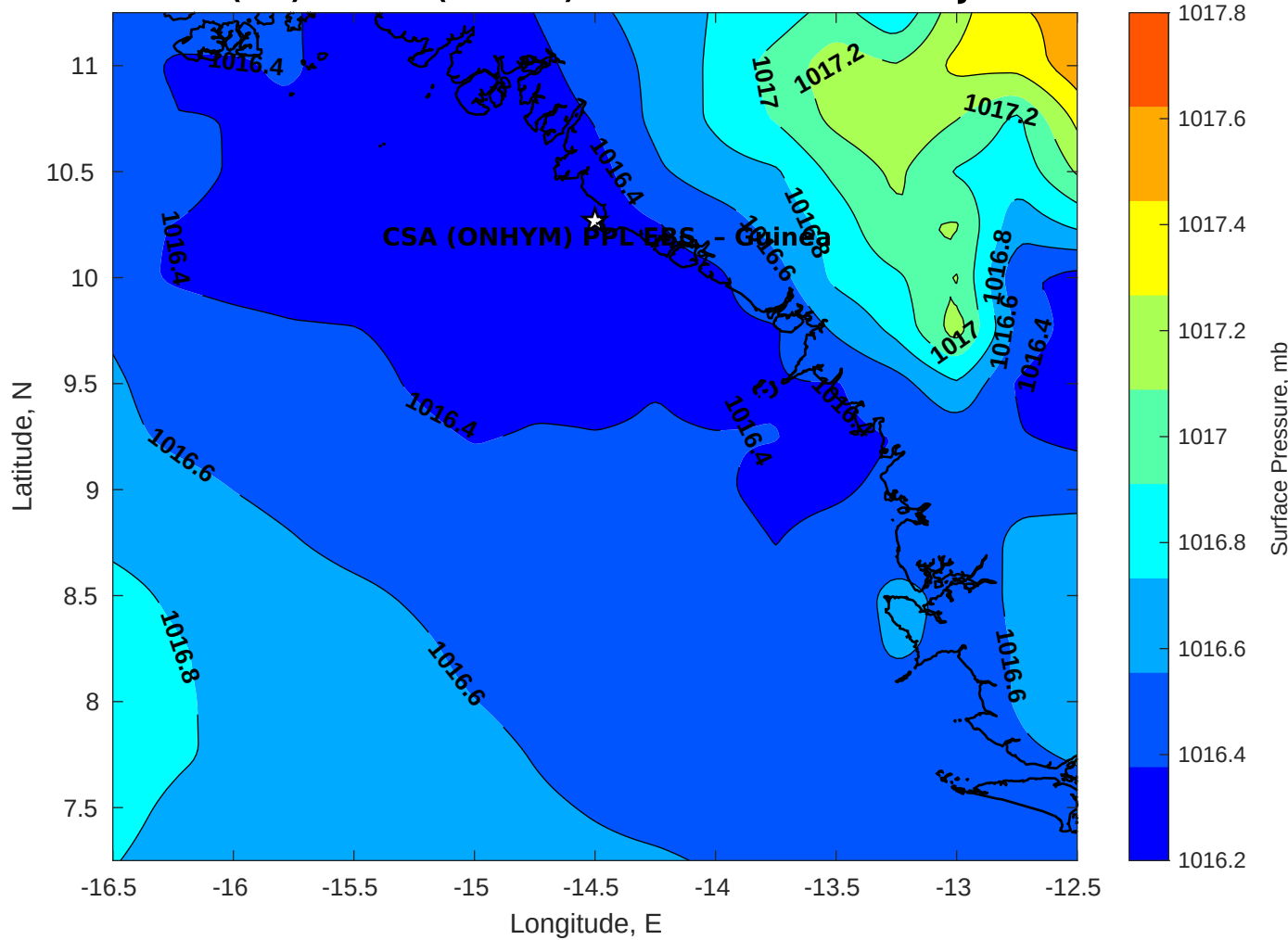
Surface Pressure (mb) for CSA (ONHYM) PPL EBS - Guinea at 20-Jul-2025 00:00:00
