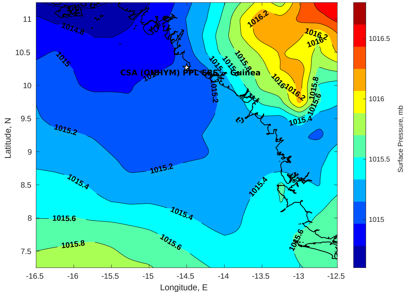
Surface Pressure (mb) for CSA (ONHYM) PPL EBS - Guinea at 21-Jul-2025 00:00:00
