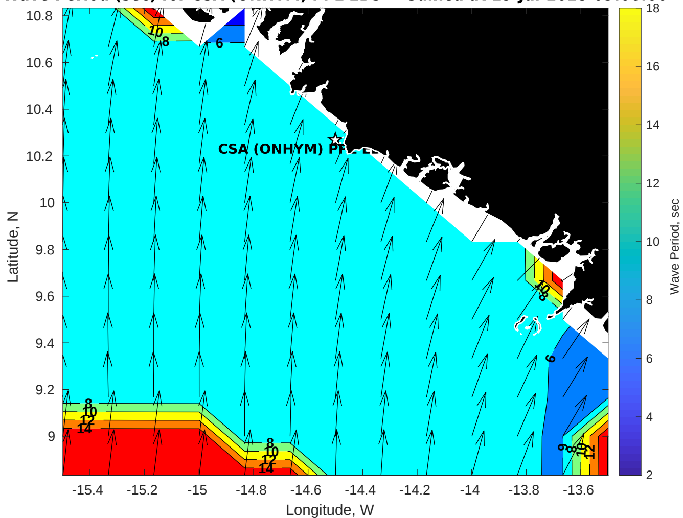
Wave Period (sec) for CSA (ONHYM) PPL EBS - Guinea at 19-Jul-2025 09:00:00
