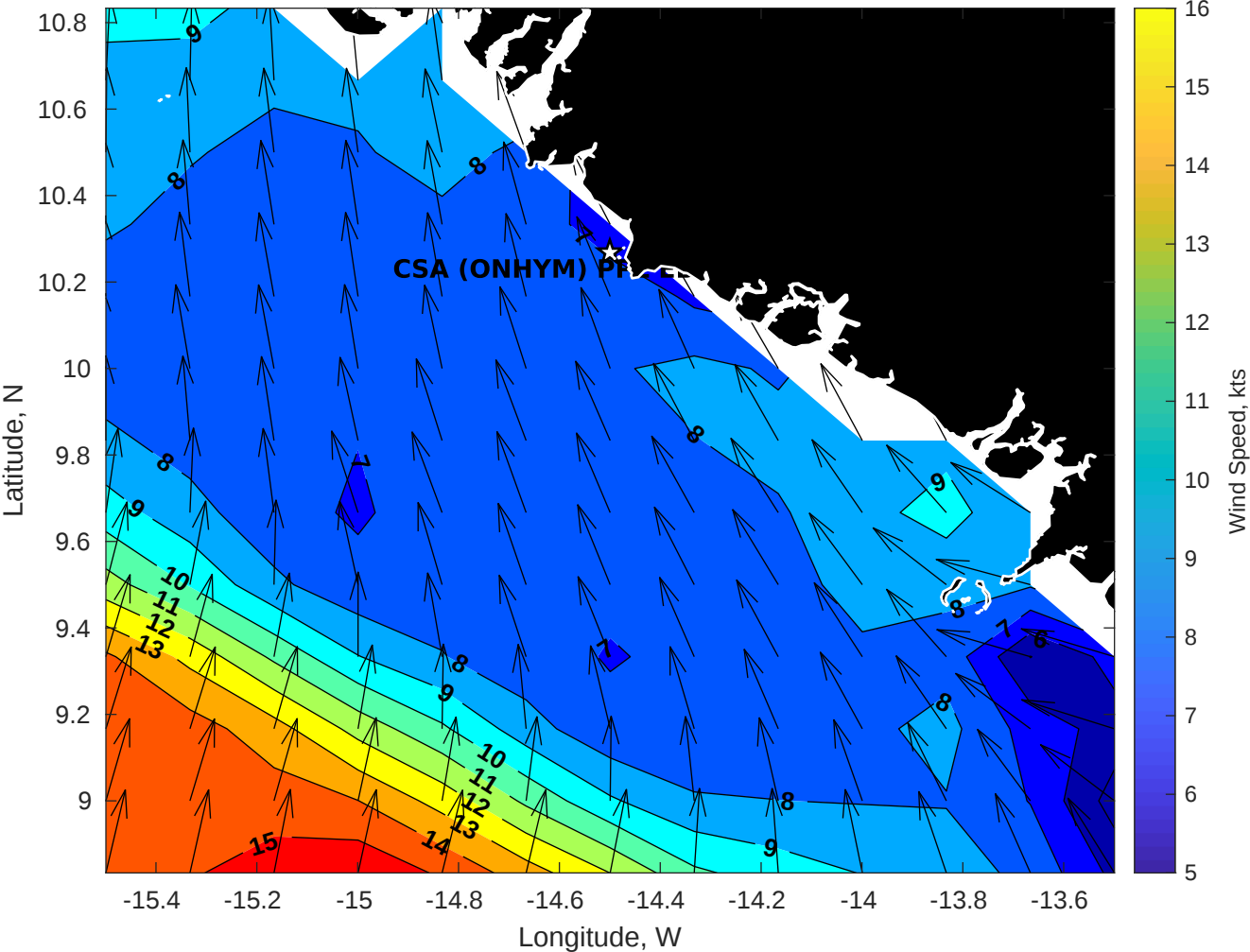
Winds (kts) for CSA (ONHYM) PPL EBS - Guinea at 19-Jul-2025 09:00:00
