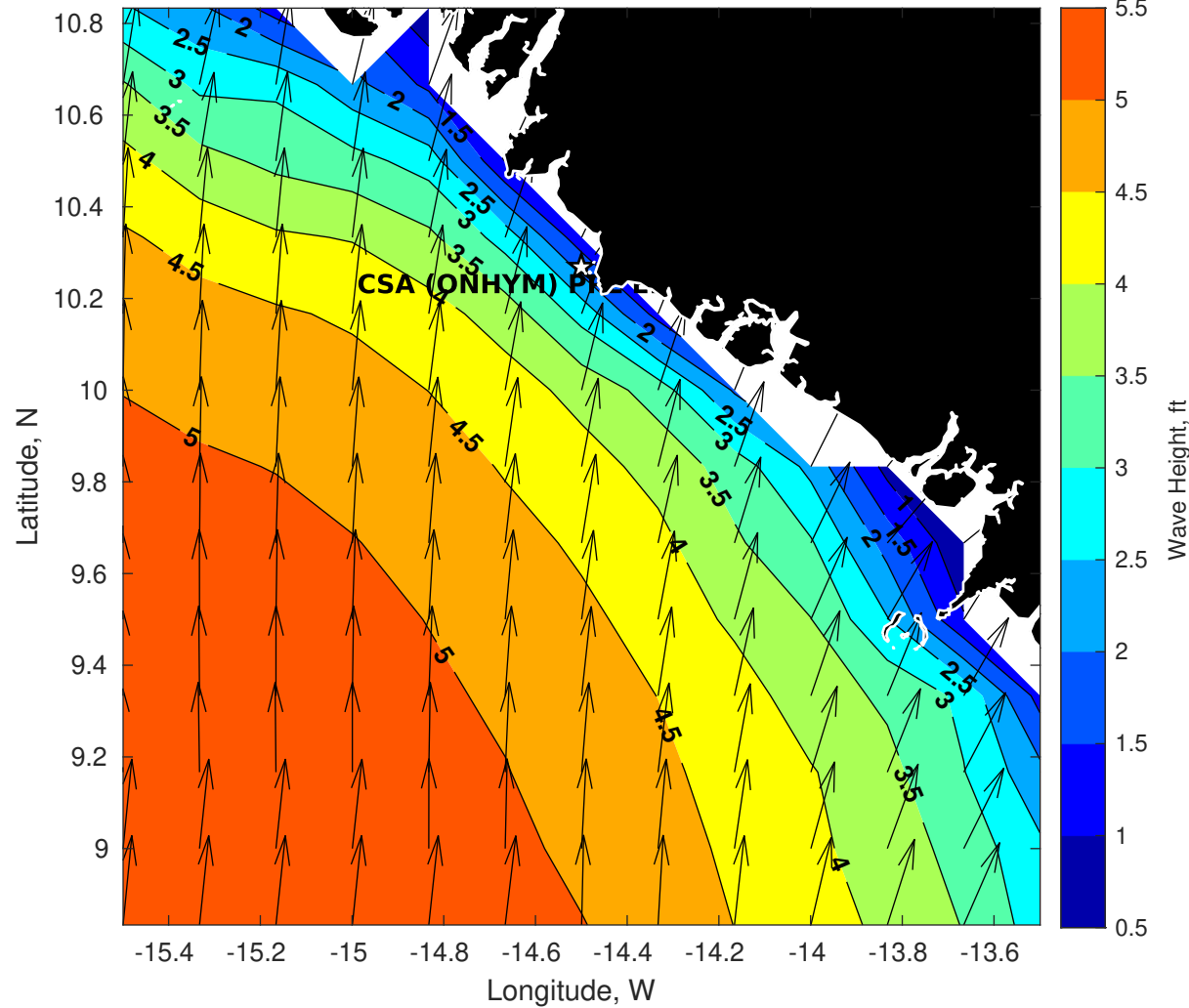
Wave Height (ft) for CSA (ONHYM) PPL EBS - Guinea at 19-Jul-2025 09:00:00
