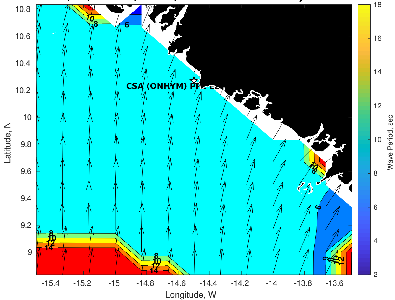
Wave Period (sec) for CSA (ONHYM) PPL EBS - Guinea at 19-Jul-2025 09:00:00
