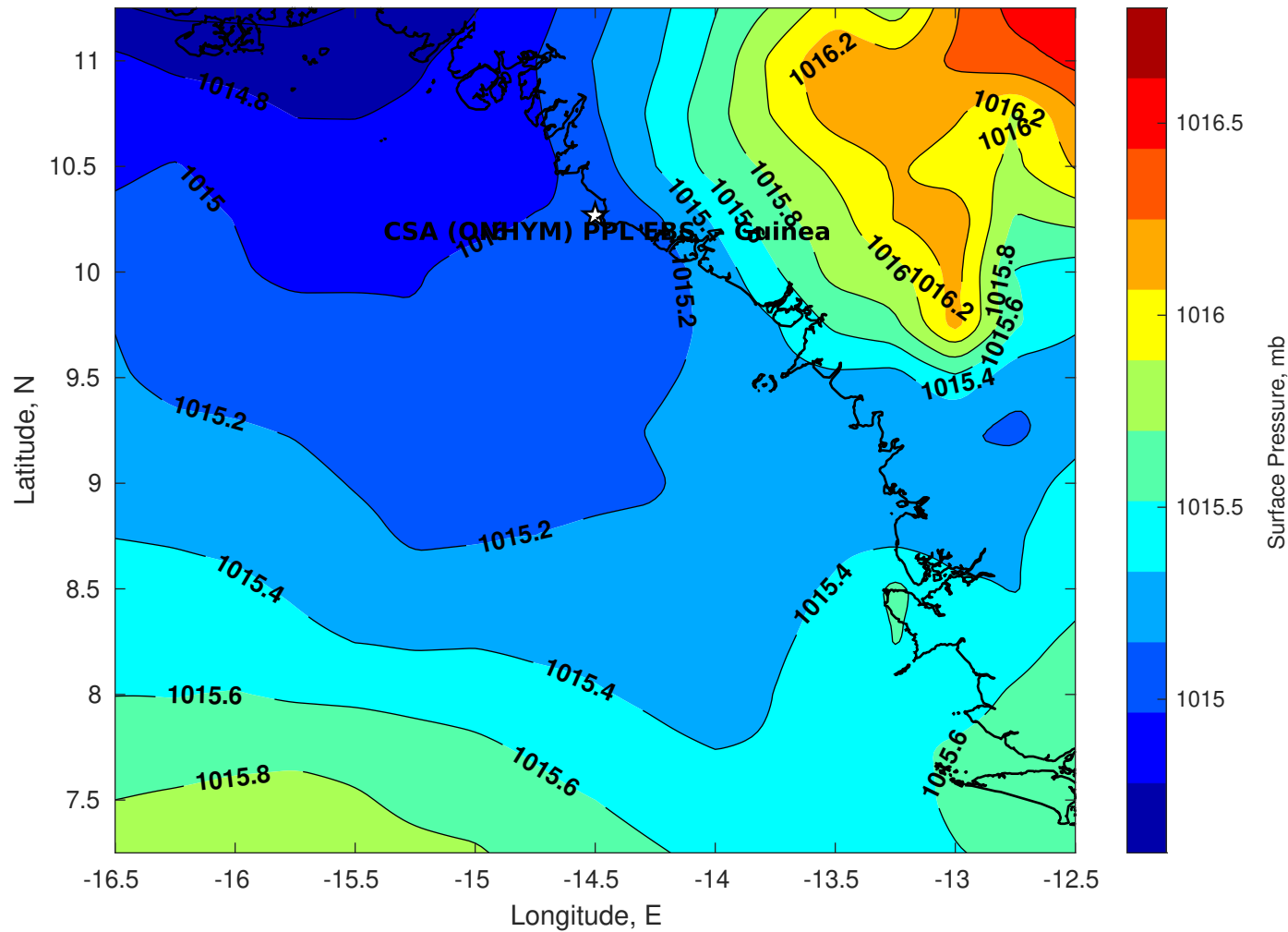
Surface Pressure (mb) for CSA (ONHYM) PPL EBS - Guinea at 21-Jul-2025 00:00:00
