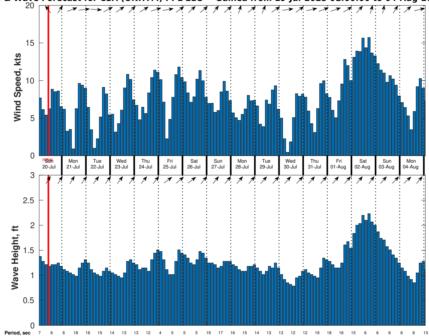
Wind & Wave Forecast for CSA (ONHYM) PPL EBS - Guinea from 19-Jul-2025 01:00:00 to 04-Aug-2025 01:00:00
