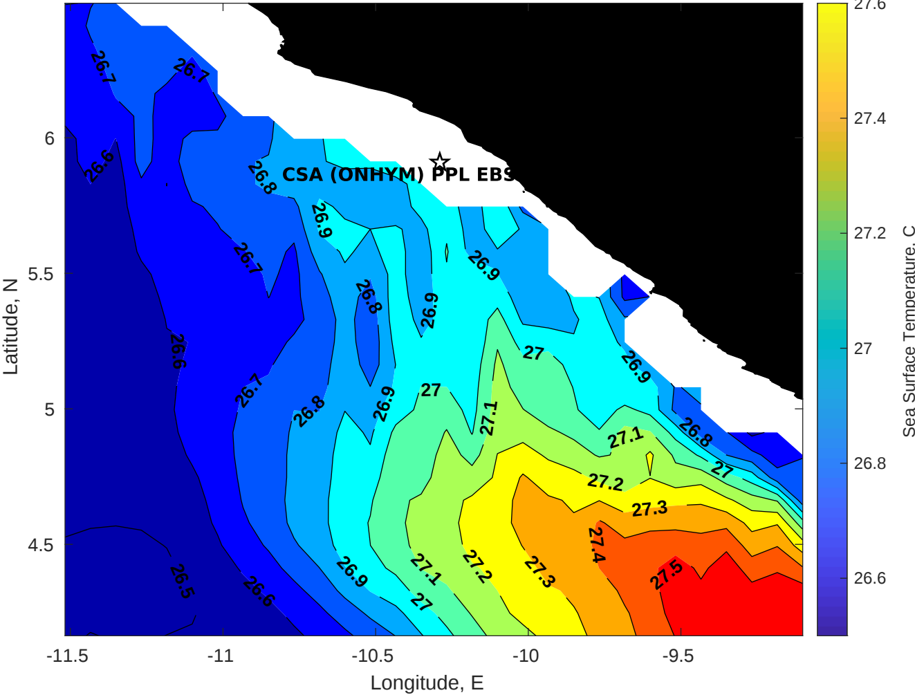
SST for CSA (ONHYM) PPL EBS - Liberia at 18-Jul-2025 00:00:00
