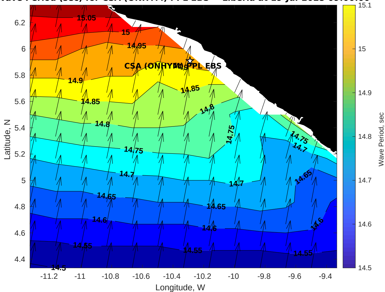
Wave Period (sec) for CSA (ONHYM) PPL EBS - Liberia at 19-Jul-2025 09:00:00
