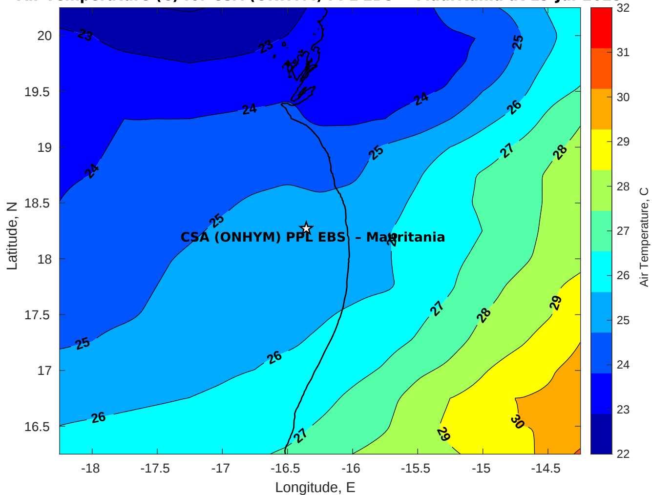
Air Temperature (C) for CSA (ONHYM) PPL EBS - Mauritania at 19-Jul-2025
