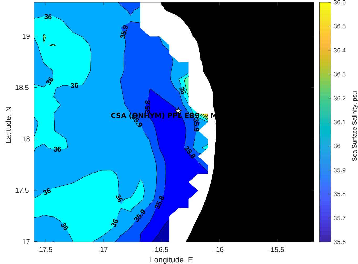
Surface Salinity for CSA (ONHYM) PPL EBS - Mauritania at 18-Jul-2025 00:00:00
