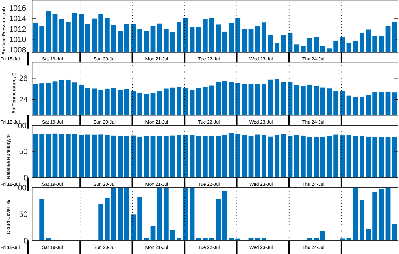
Met Forecast for CSA (ONHYM) PPL EBS - Mauritania from 19-Jul-2025 00:00:00 to 26-Jul-2025 00:00:00
