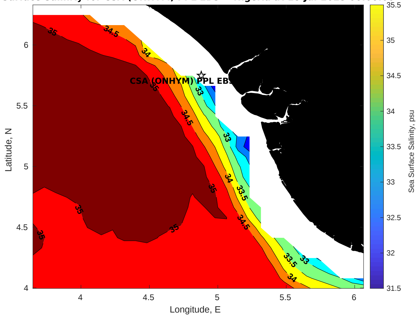
Surface Salinity for CSA (ONHYM) PPL EBS - Nigeria at 18-Jul-2025 00:00:00
