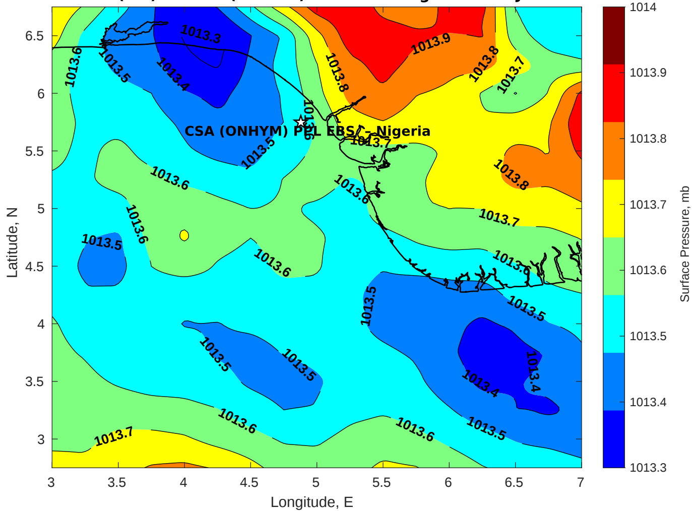
Surface Pressure (mb) for CSA (ONHYM) PPL EBS - Nigeria at 21-Jul-2025 00:00:00
