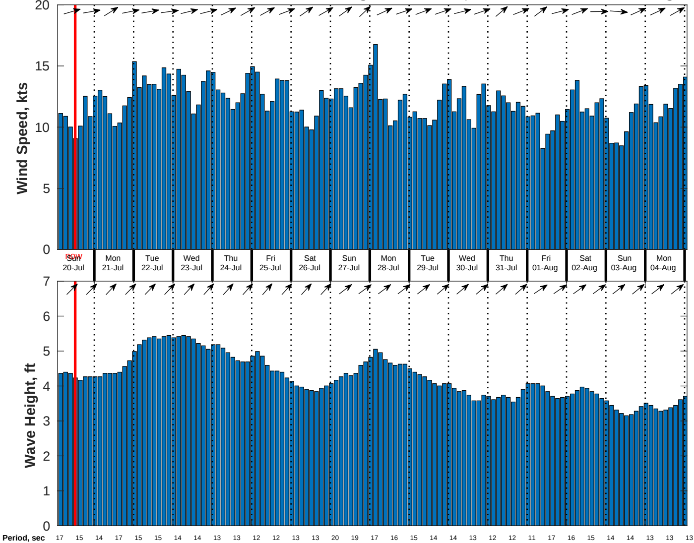
Wind & Wave Forecast for CSA (ONHYM) PPL EBS - Nigeria from 19-Jul-2025 02:00:00 to 04-Aug-2025 02:00:00
