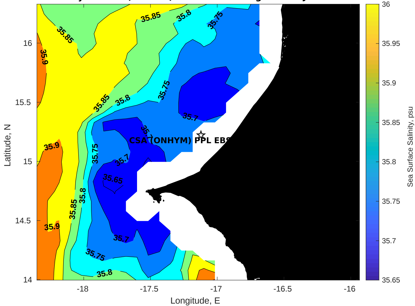
Surface Salinity for CSA (ONHYM) PPL EBS - Senegal at 18-Jul-2025 00:00:00
