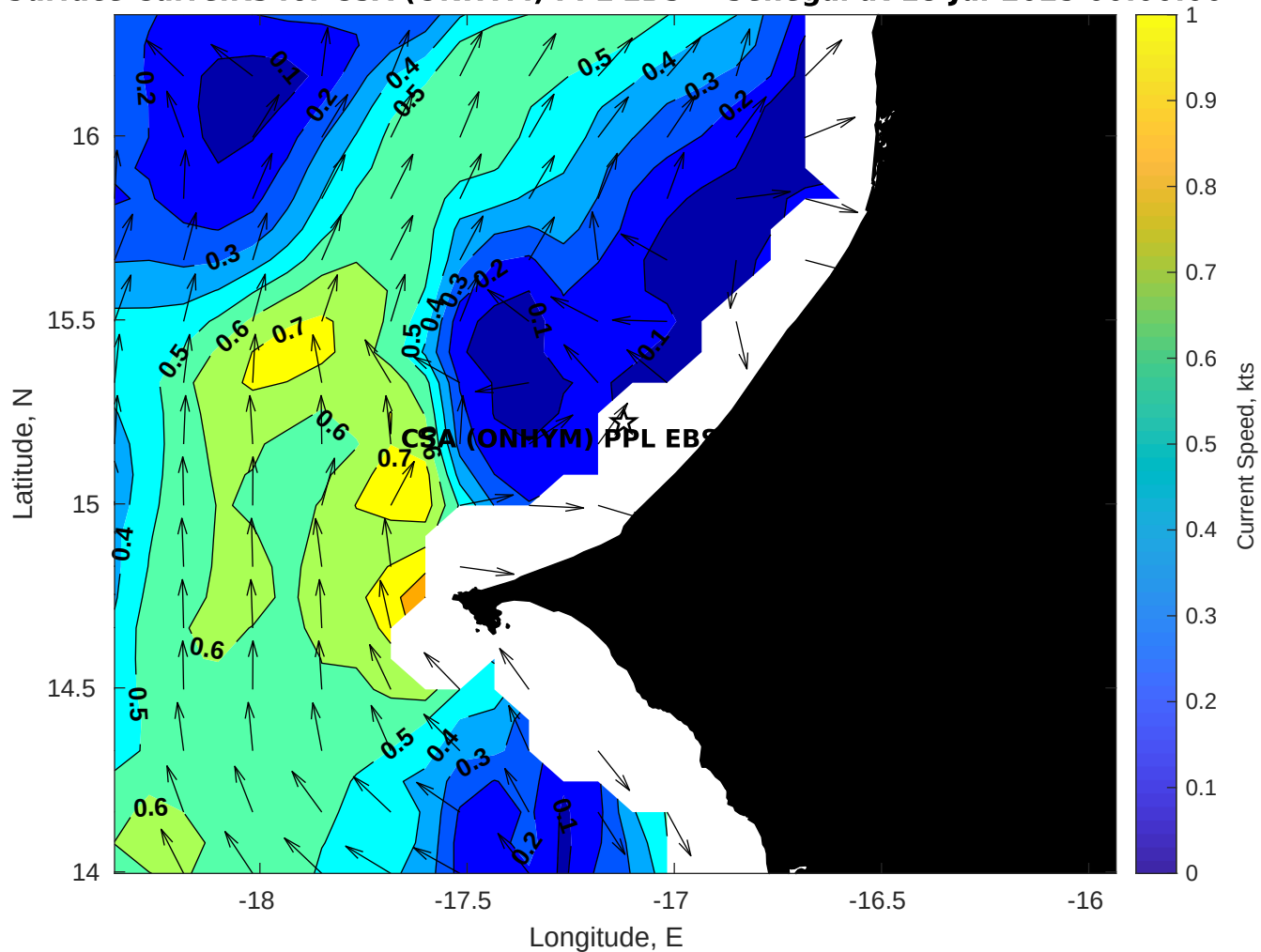
Surface Currents for CSA (ONHYM) PPL EBS - Senegal at 18-Jul-2025 00:00:00
