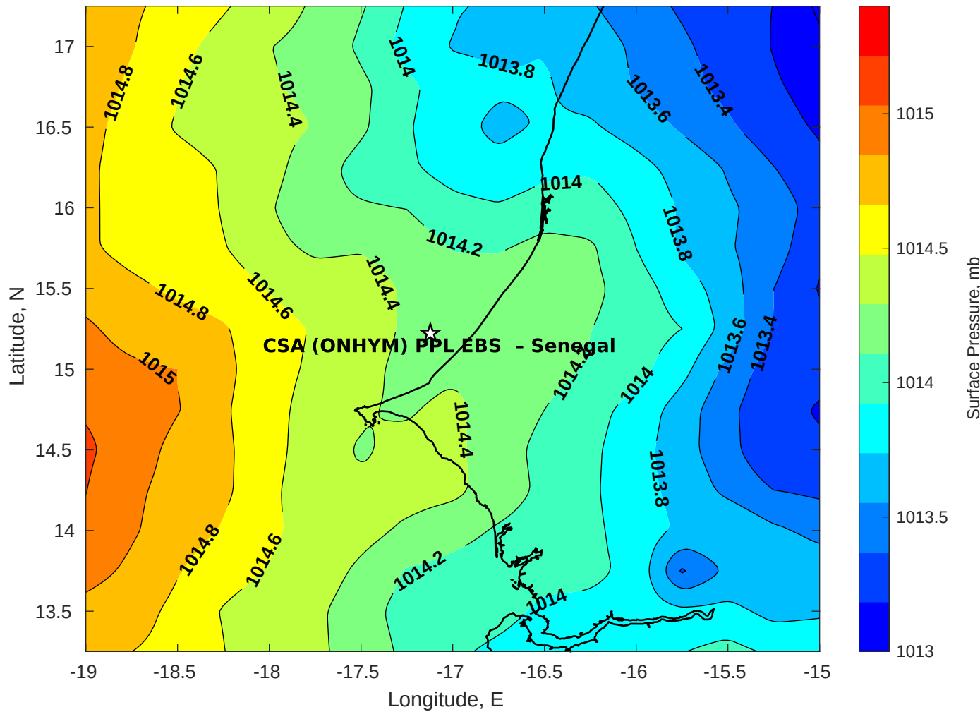
Surface Pressure (mb) for CSA (ONHYM) PPL EBS - Senegal at 21-Jul-2025 00:00:00
