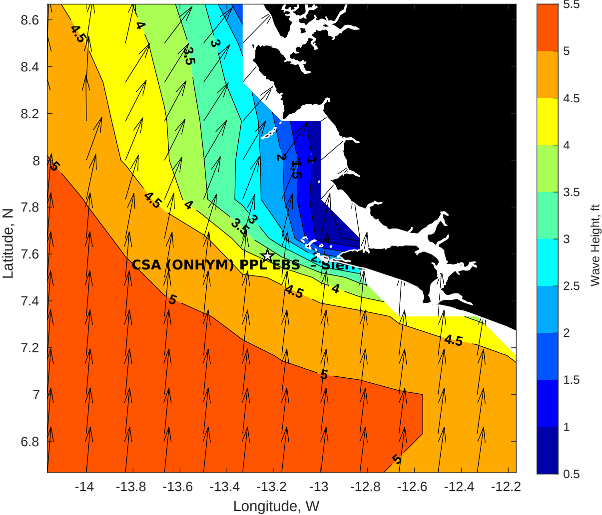
Wave Height (ft) for CSA (ONHYM) PPL EBS - Sierra Leone at 19-Jul-2025 09:00:00
