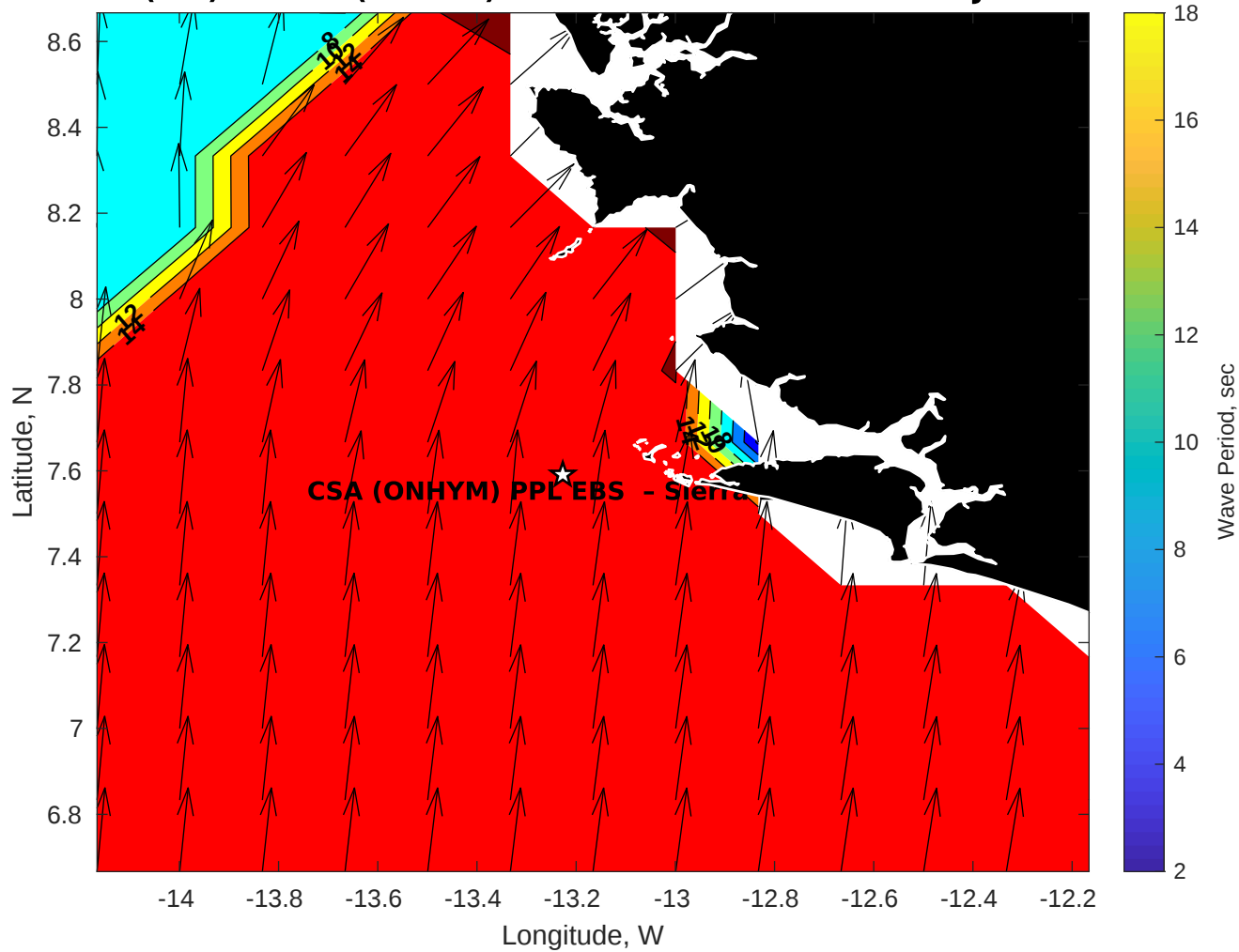
Wave Period (sec) for CSA (ONHYM) PPL EBS - Sierra Leone at 19-Jul-2025 09:00:00
