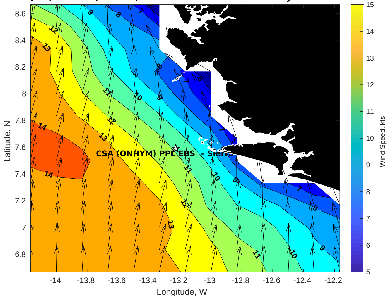
Winds (kts) for CSA (ONHYM) PPL EBS - Sierra Leone at 19-Jul-2025 09:00:00
