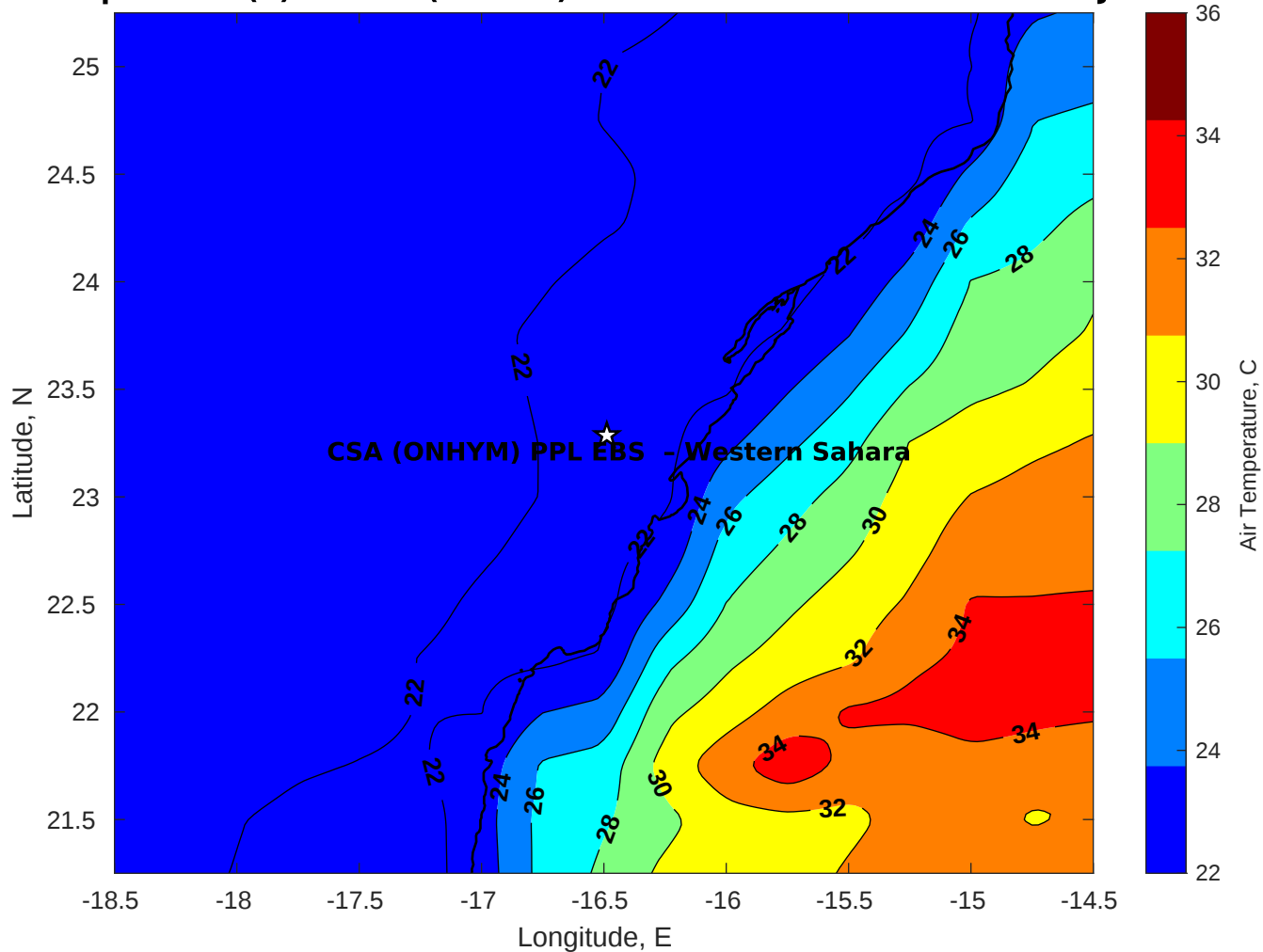
Air Temperature (C) for CSA (ONHYM) PPL EBS - Western Sahara at 19-Jul-2025
