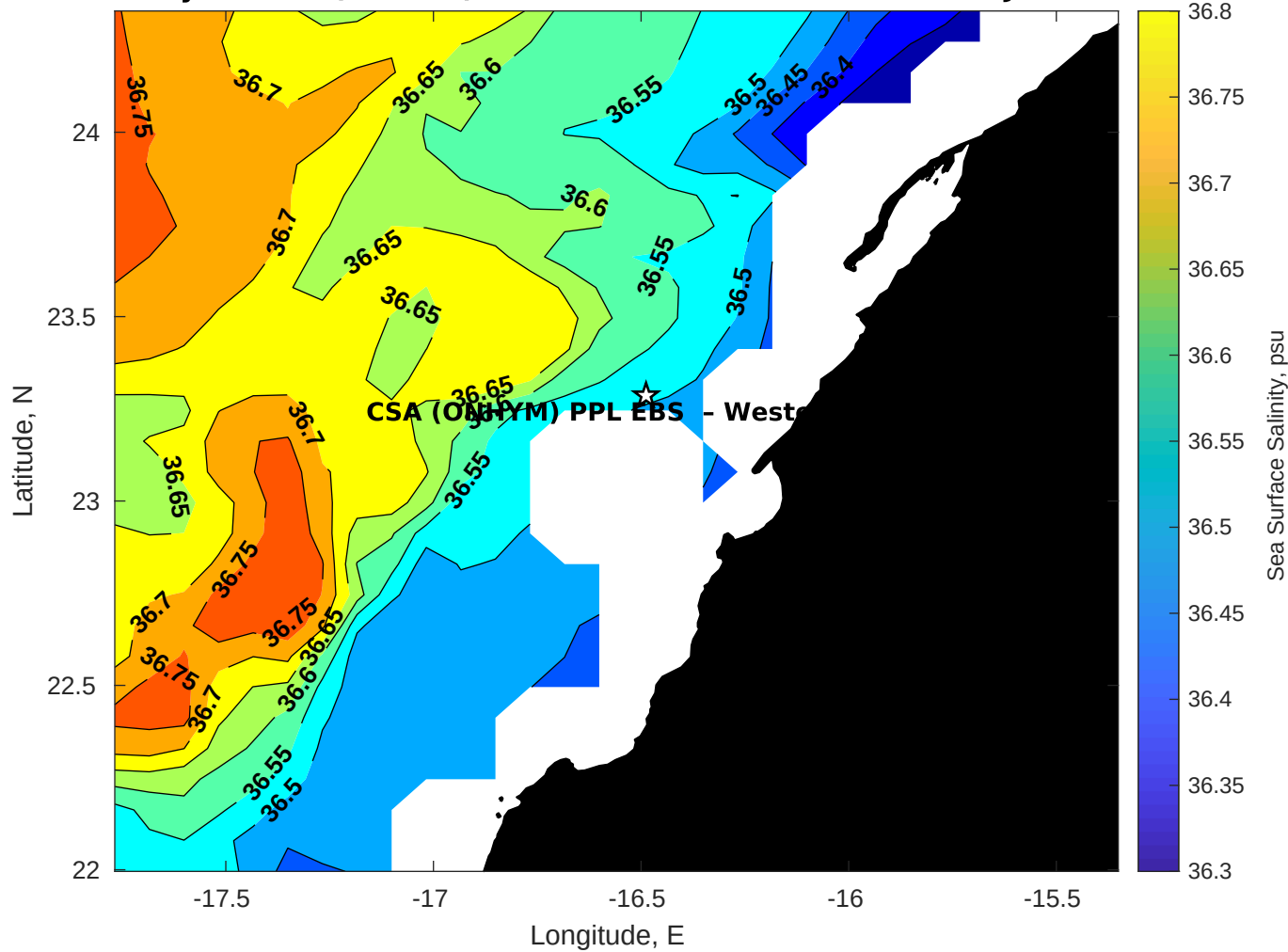
Surface Salinity for CSA (ONHYM) PPL EBS - Western Sahara at 18-Jul-2025 00:00:00
