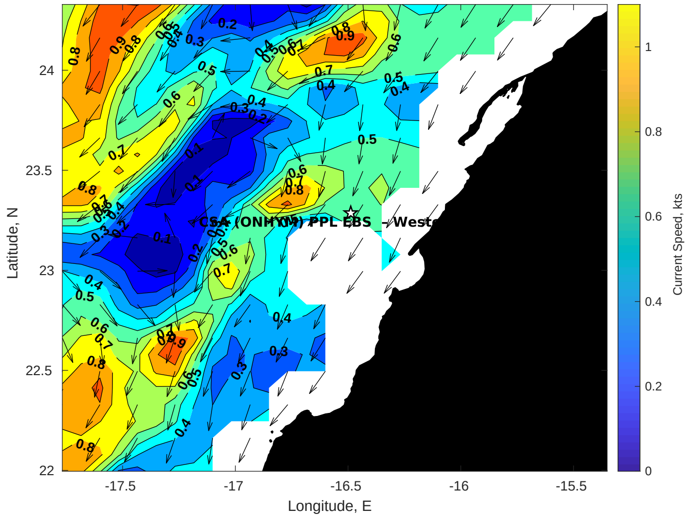
Surface Currents for CSA (ONHYM) PPL EBS - Western Sahara at 18-Jul-2025 00:00:00
