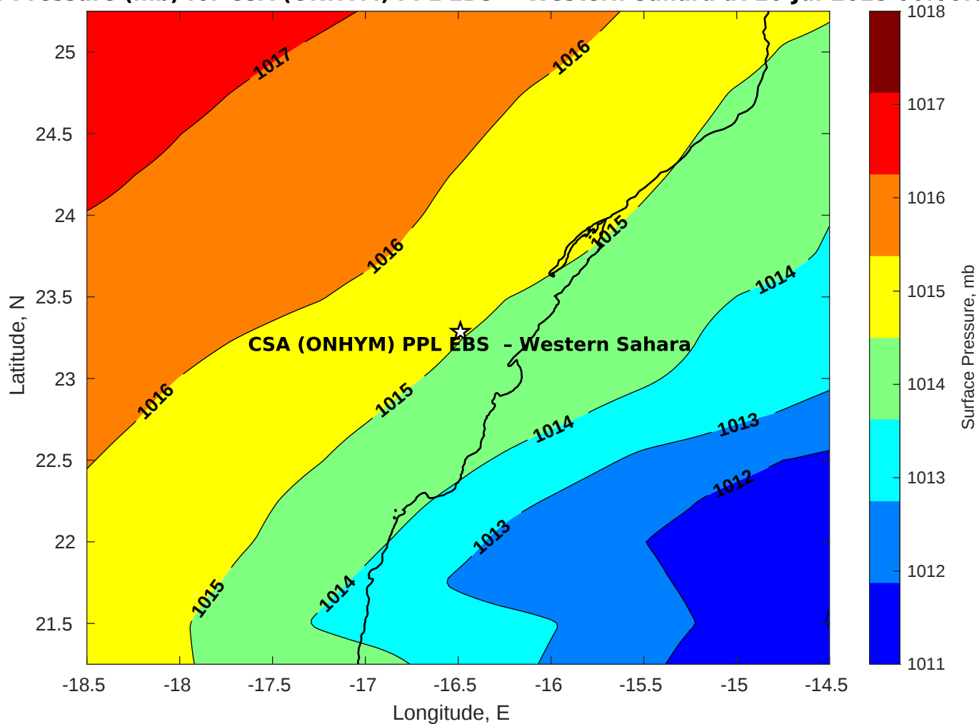
Surface Pressure (mb) for CSA (ONHYM) PPL EBS - Western Sahara at 20-Jul-2025 00:00:00
