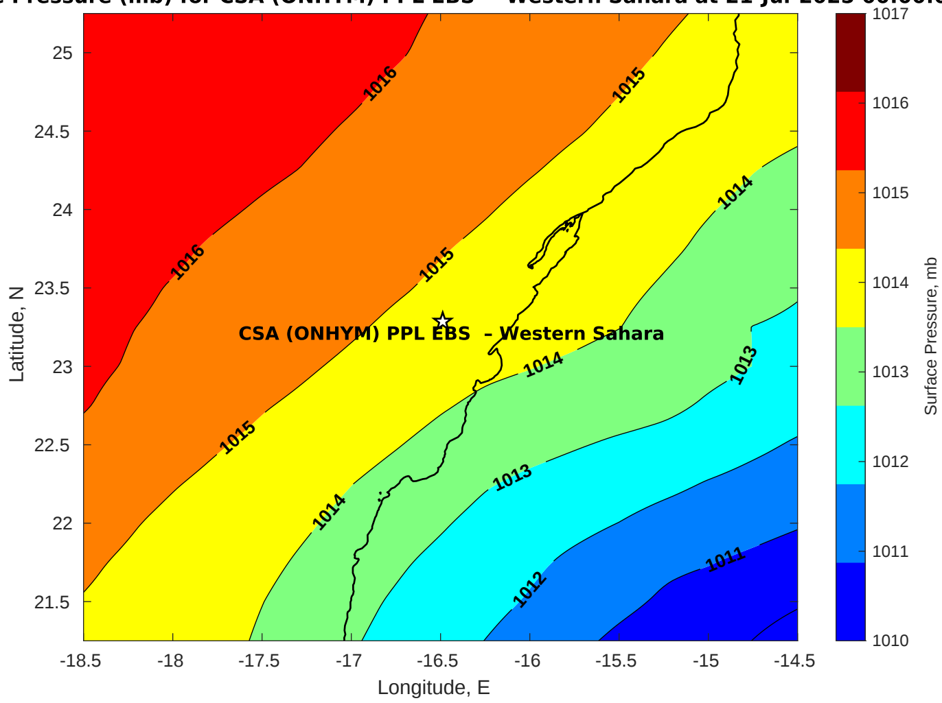
Surface Pressure (mb) for CSA (ONHYM) PPL EBS - Western Sahara at 21-Jul-2025 00:00:00
