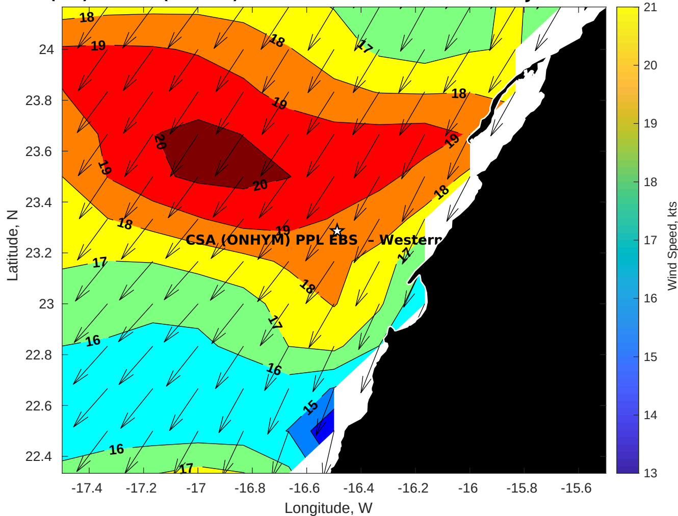
Winds (kts) for CSA (ONHYM) PPL EBS - Western Sahara at 19-Jul-2025 09:00:00
