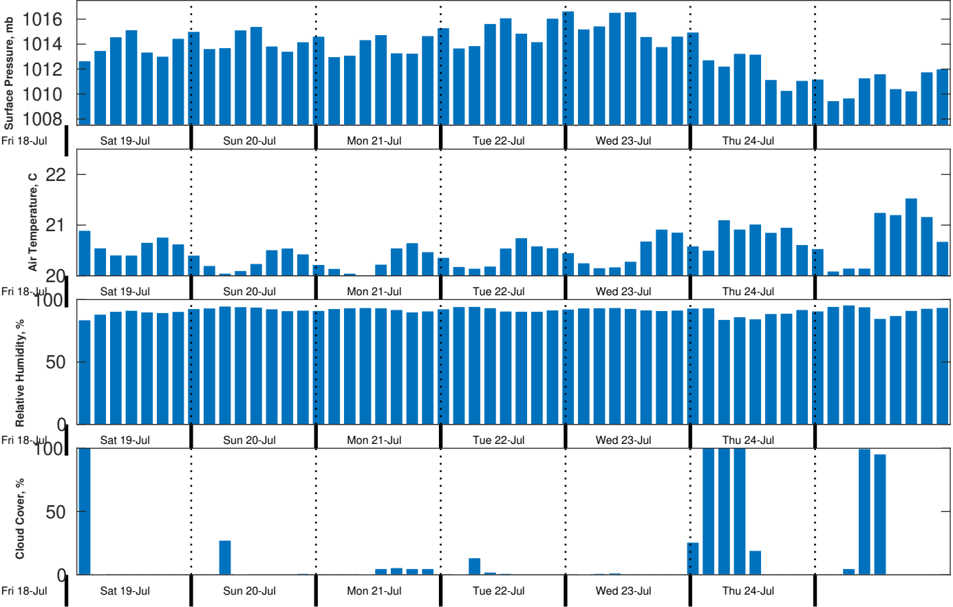
Met Forecast for CSA (ONHYM) PPL EBS - Western Sahara from 19-Jul-2025 00:00:00 to 26-Jul-2025 00:00:00
