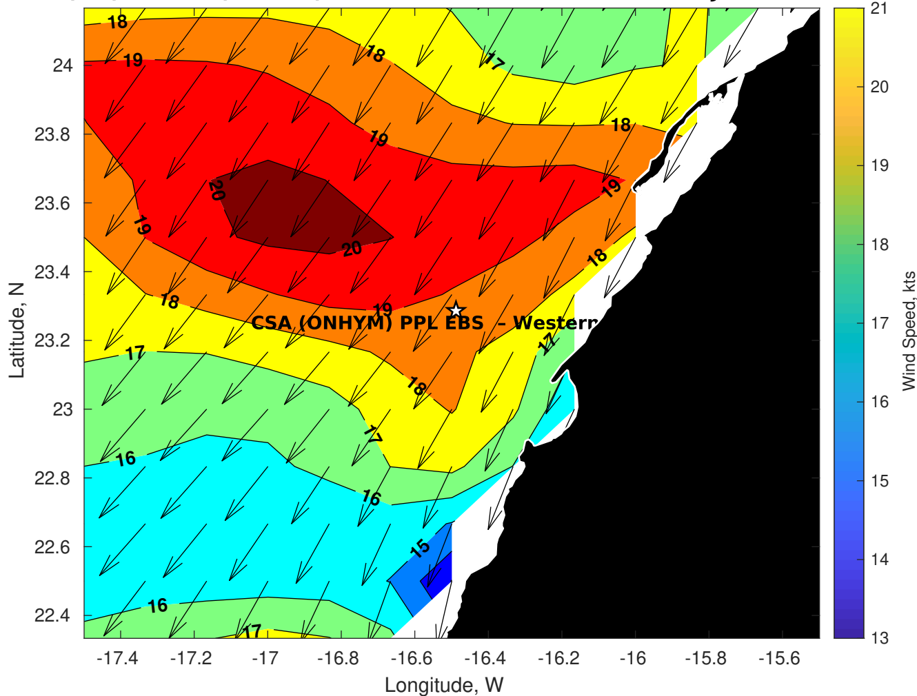
Winds (kts) for CSA (ONHYM) PPL EBS - Western Sahara at 19-Jul-2025 09:00:00
