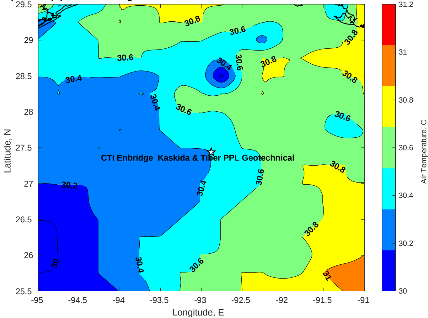
Air Temperature (C) for CTI Enbridge Kaskida & Tiber PPL Geotechnical at 19-Jul-2025
