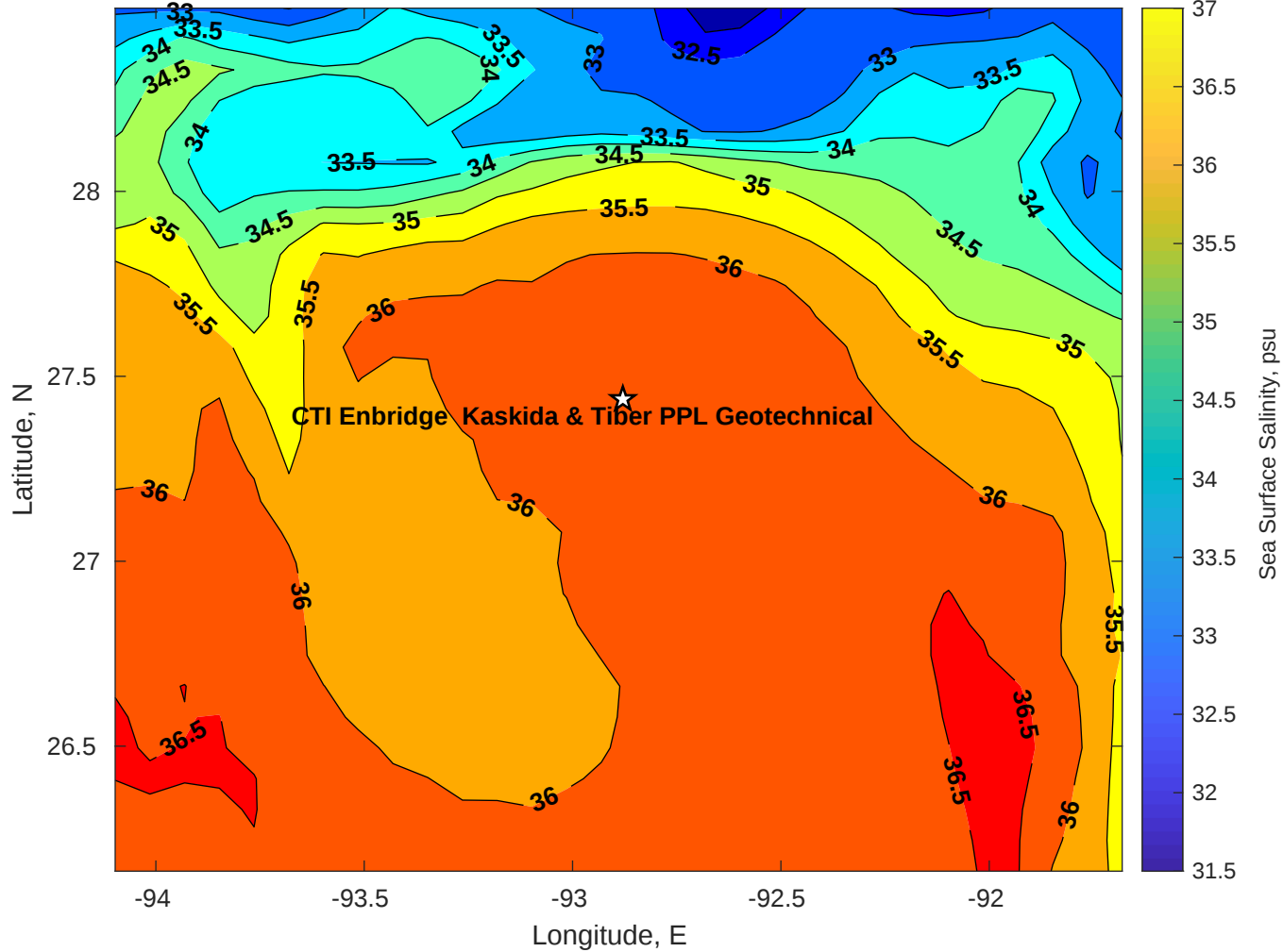
Surface Salinity for CTI Enbridge Kaskida & Tiber PPL Geotechnical at 18-Jul-2025 00:00:00
