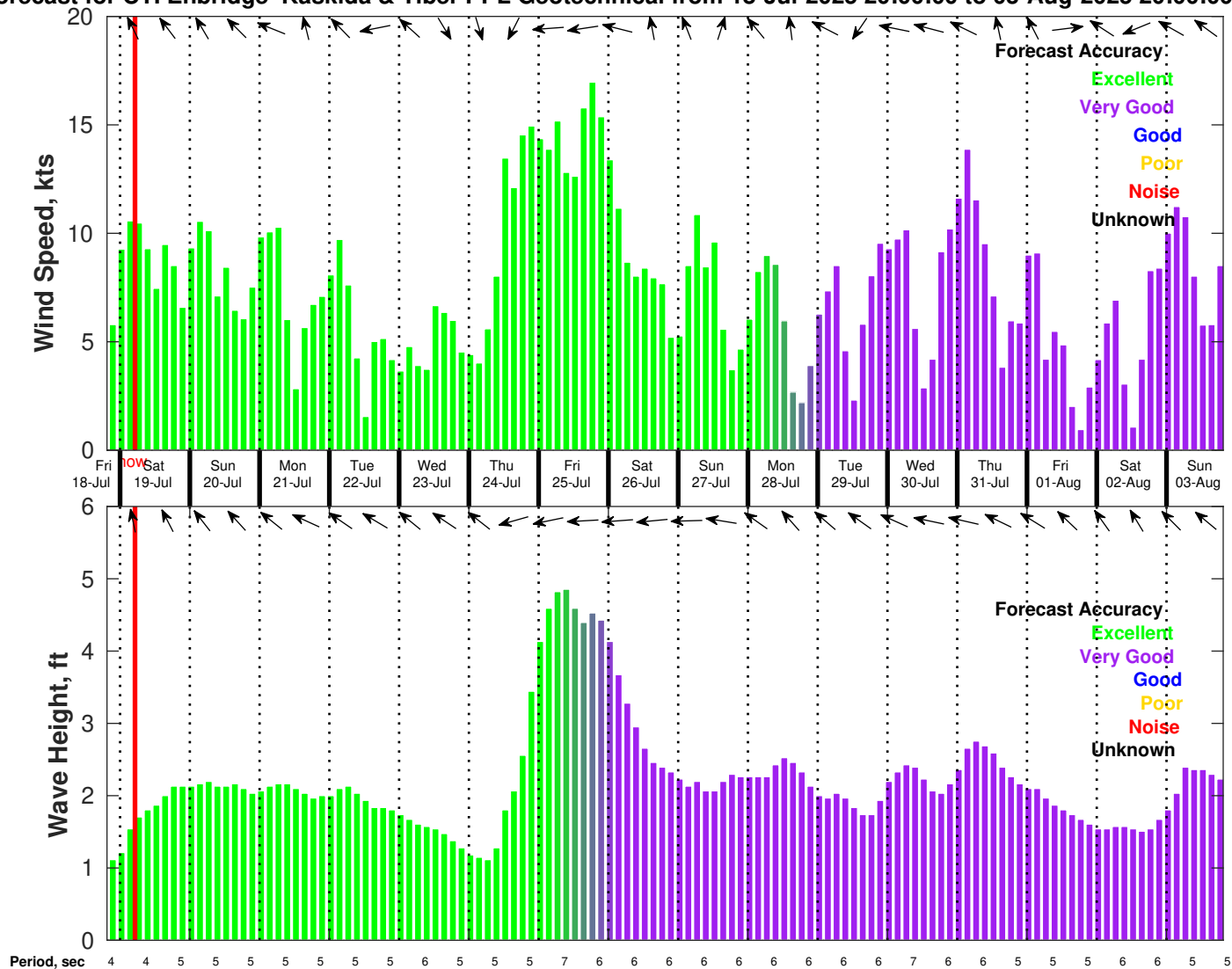
Wind & Wave Forecast for CTI Enbridge Kaskida & Tiber PPL Geotechnical from 18-Jul-2025 20:00:00 to 03-Aug-2025 20:00:00
