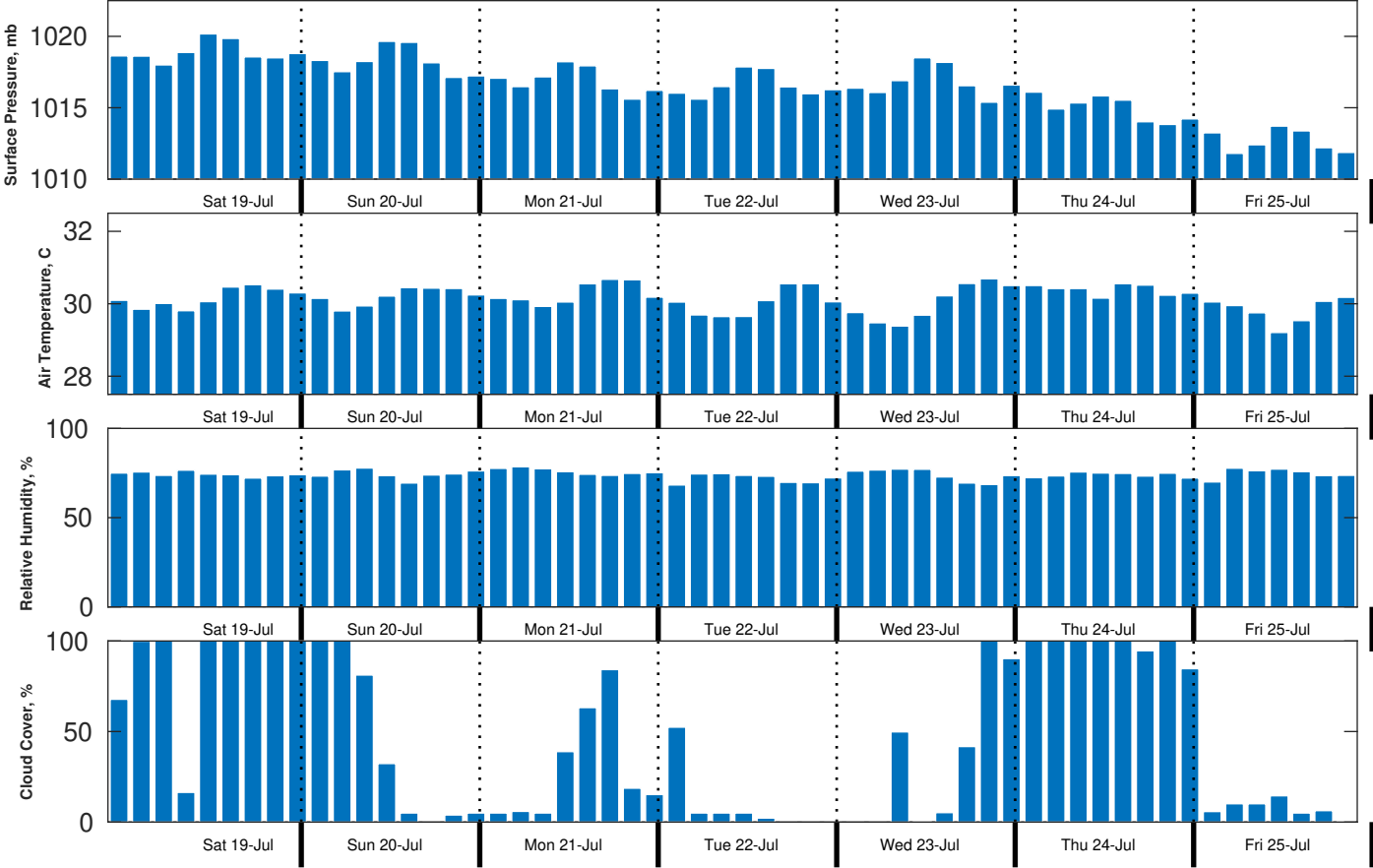
Met Forecast for CTI Enbridge Kaskida & Tiber PPL Geotechnical from 19-Jul-2025 00:00:00 to 26-Jul-2025 00:00:00
