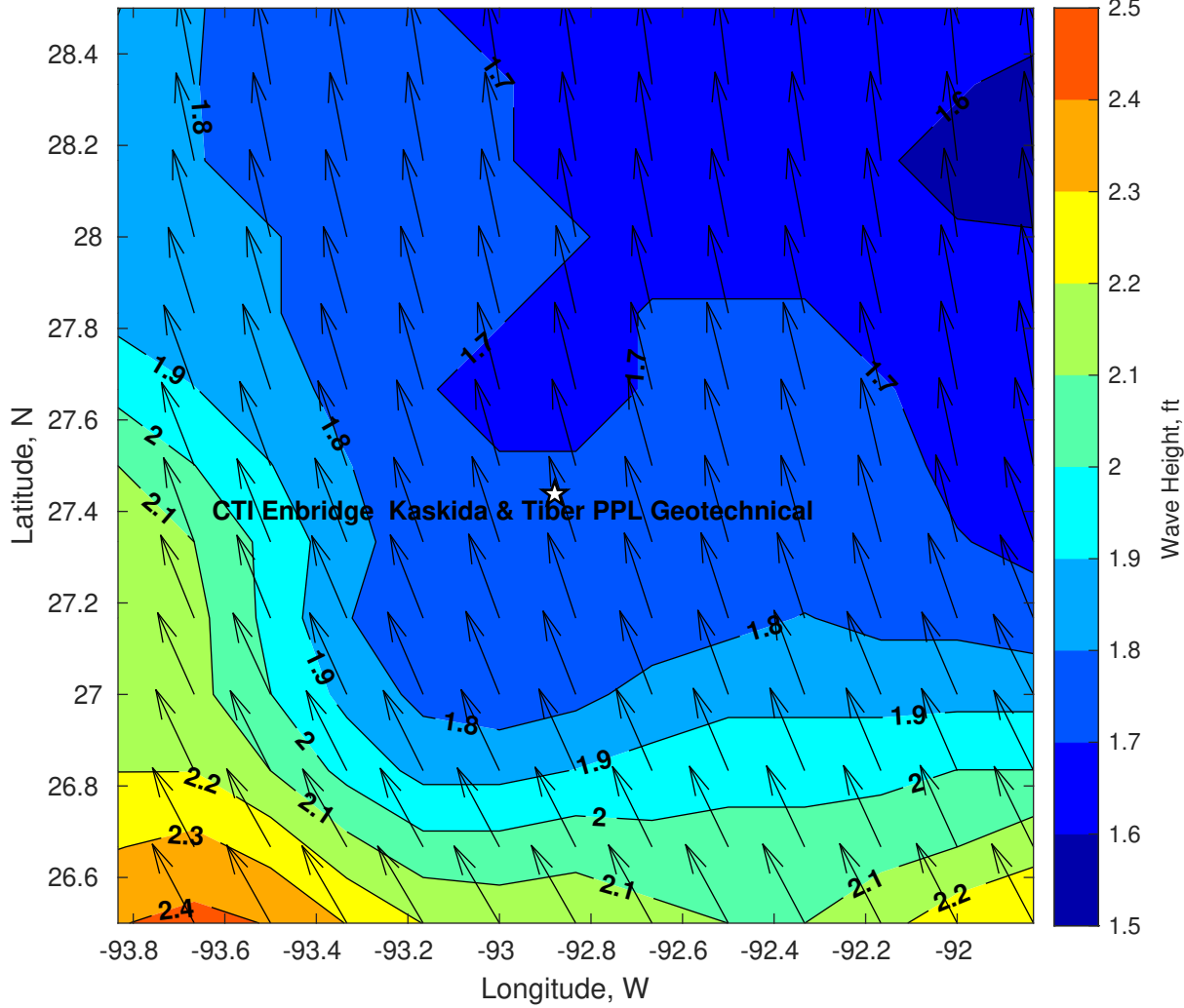
Wave Height (ft) for CTI Enbridge Kaskida & Tiber PPL Geotechnical at 19-Jul-2025 09:00:00
