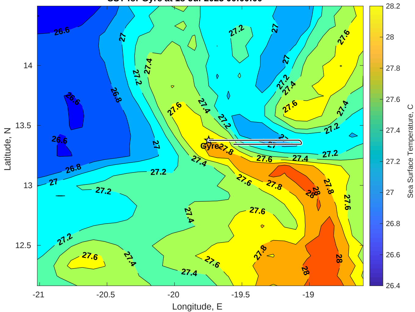
SST for Gyre at 18-Jul-2025 00:00:00
