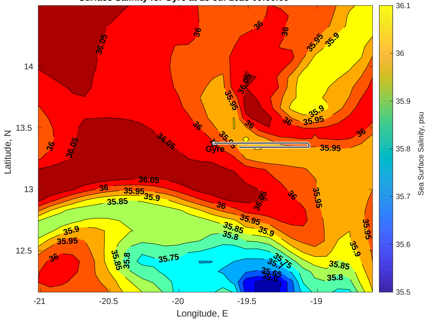
Surface Salinity for Gyre at 18-Jul-2025 00:00:00
