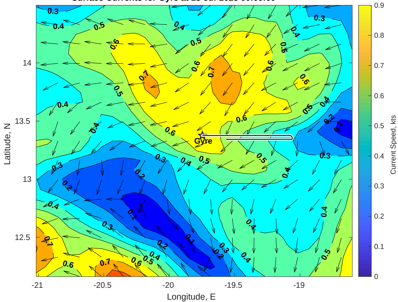
Surface Currents for Gyre at 18-Jul-2025 00:00:00
