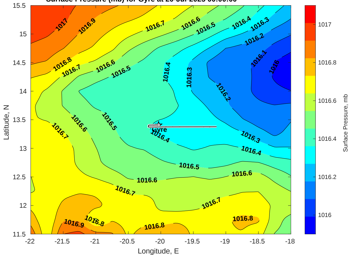
Surface Pressure (mb) for Gyre at 20-Jul-2025 00:00:00
