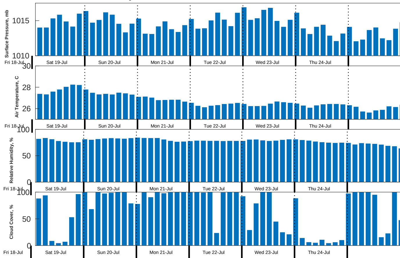
Met Forecast for Gyre from 18-Jul-2025 23:00:00 to 25-Jul-2025 23:00:00
