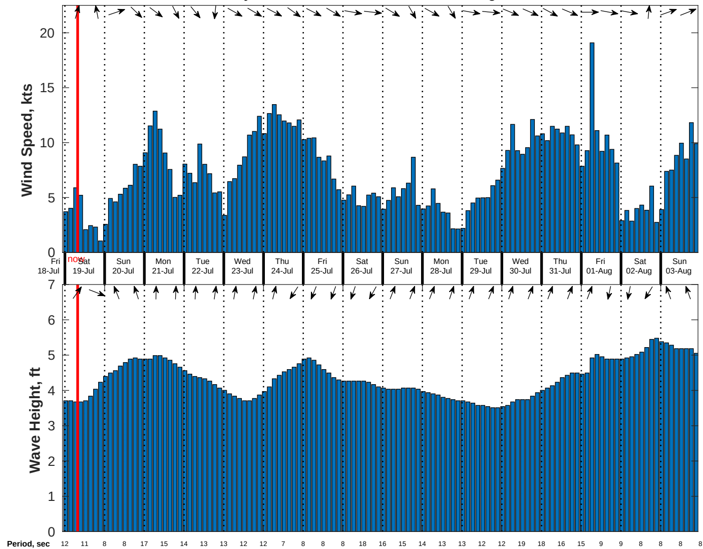
Wind & Wave Forecast for Gyre from 18-Jul-2025 23:00:00 to 03-Aug-2025 23:00:00
