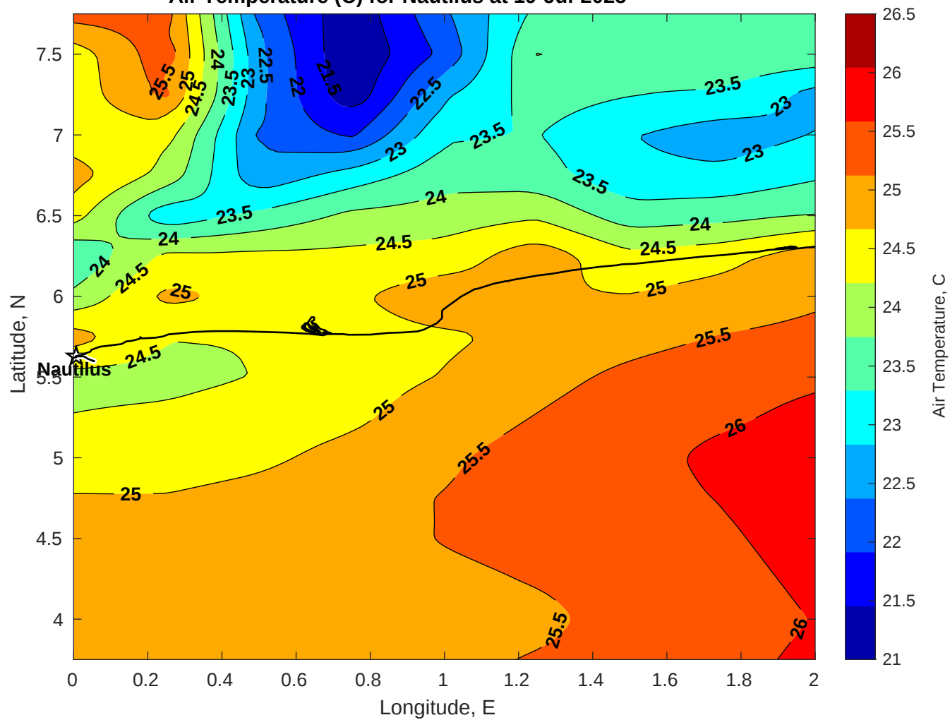
Air Temperature (C) for Nautilus at 19-Jul-2025
