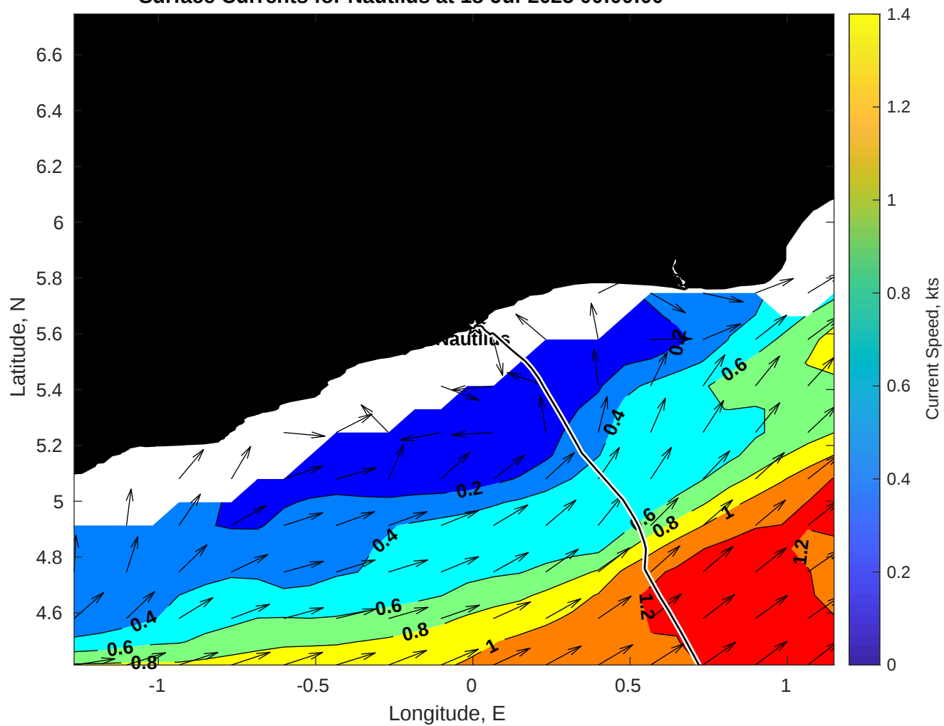
Surface Currents for Nautilus at 18-Jul-2025 00:00:00
