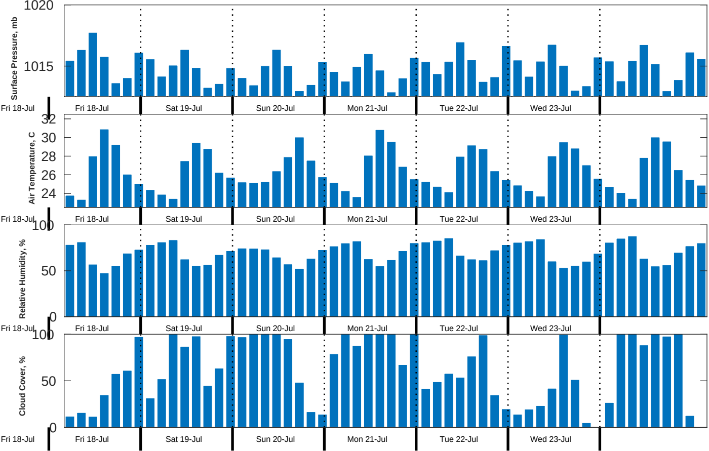
Met Forecast for Nautilus from 19-Jul-2025 00:00:00 to 26-Jul-2025 00:00:00
