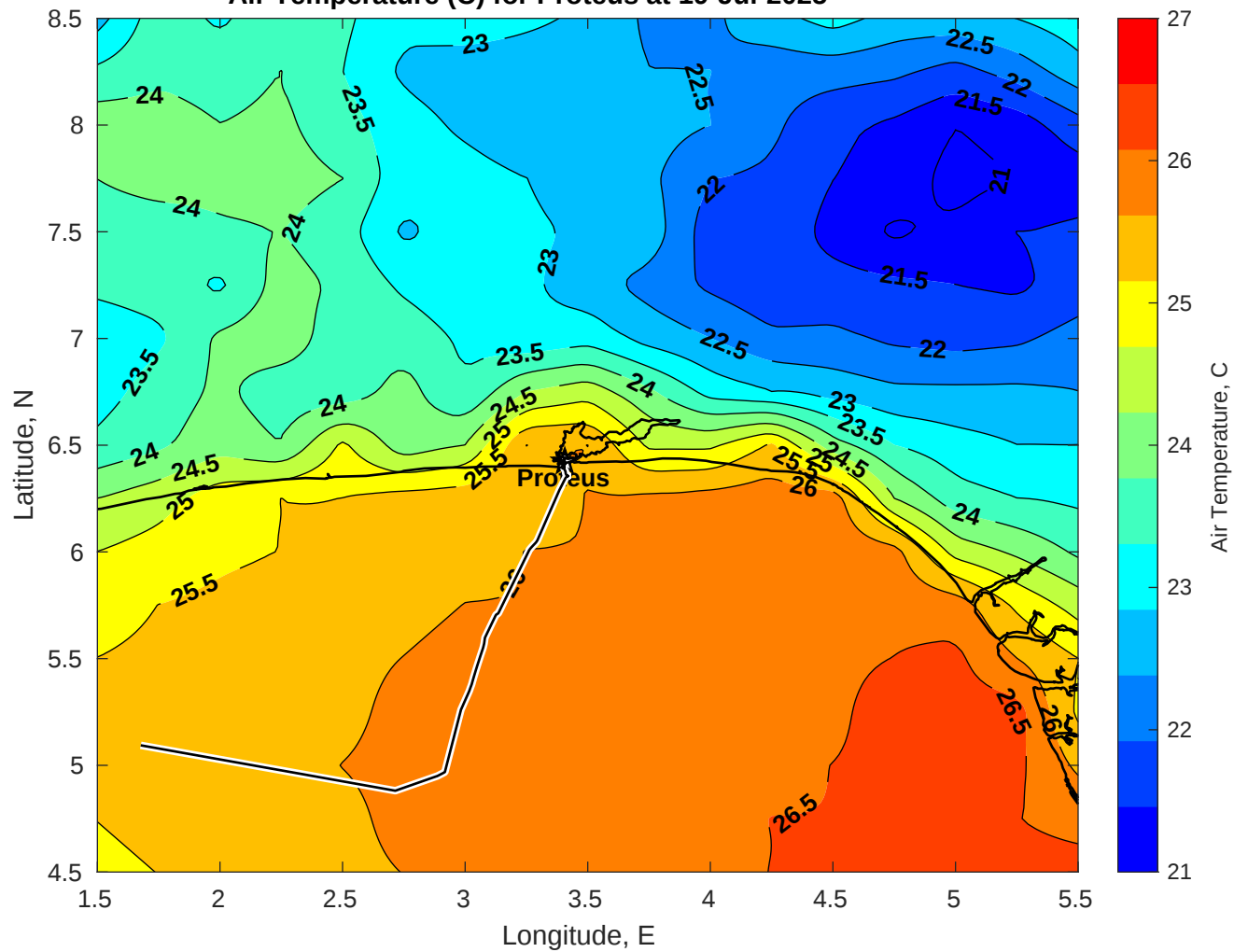
Air Temperature (C) for Proteus at 19-Jul-2025
