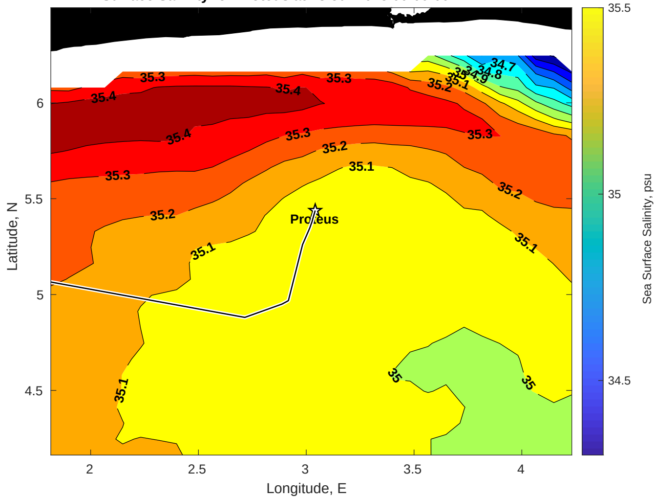
Surface Salinity for Proteus at 18-Jul-2025 00:00:00
