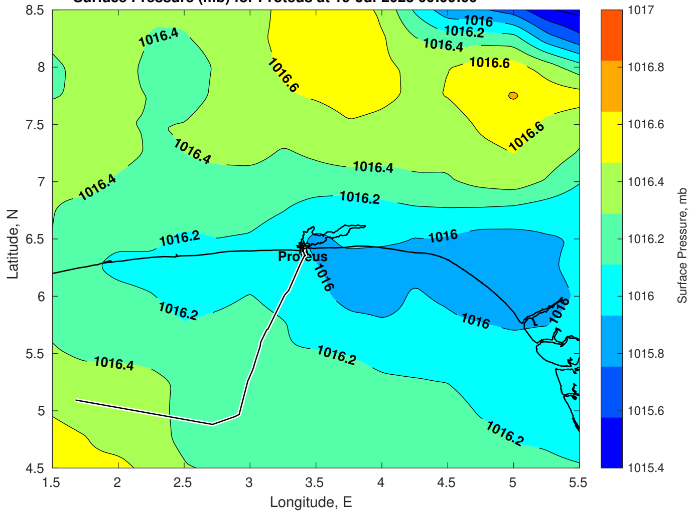
Surface Pressure (mb) for Proteus at 19-Jul-2025 00:00:00
