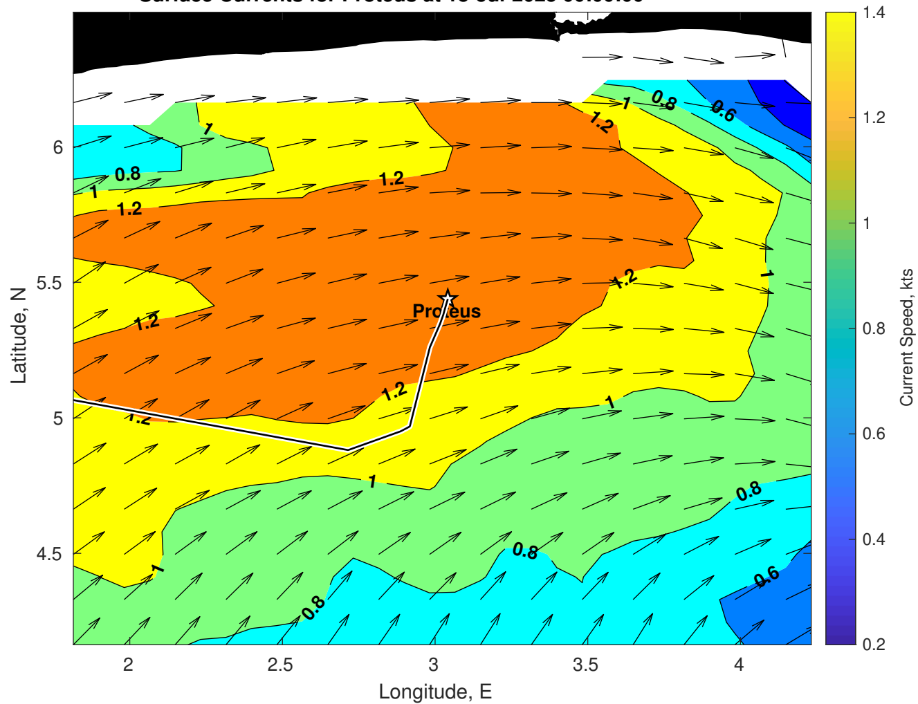
Surface Currents for Proteus at 18-Jul-2025 00:00:00
