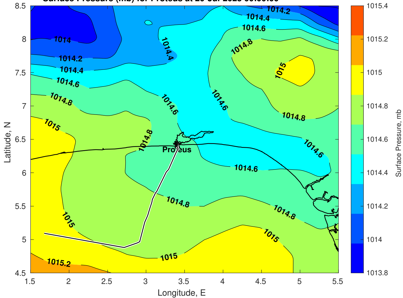
Surface Pressure (mb) for Proteus at 20-Jul-2025 00:00:00
