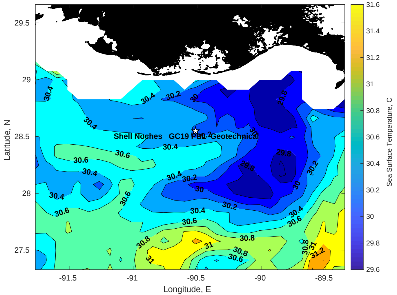
SST for Shell Noches GC19 PPL Geotechnical at 18-Jul-2025 00:00:00
