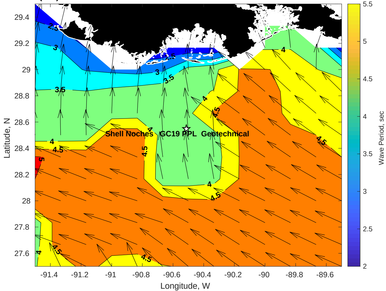
Wave Period (sec) for Shell Noches GC19 PPL Geotechnical at 19-Jul-2025 09:00:00
