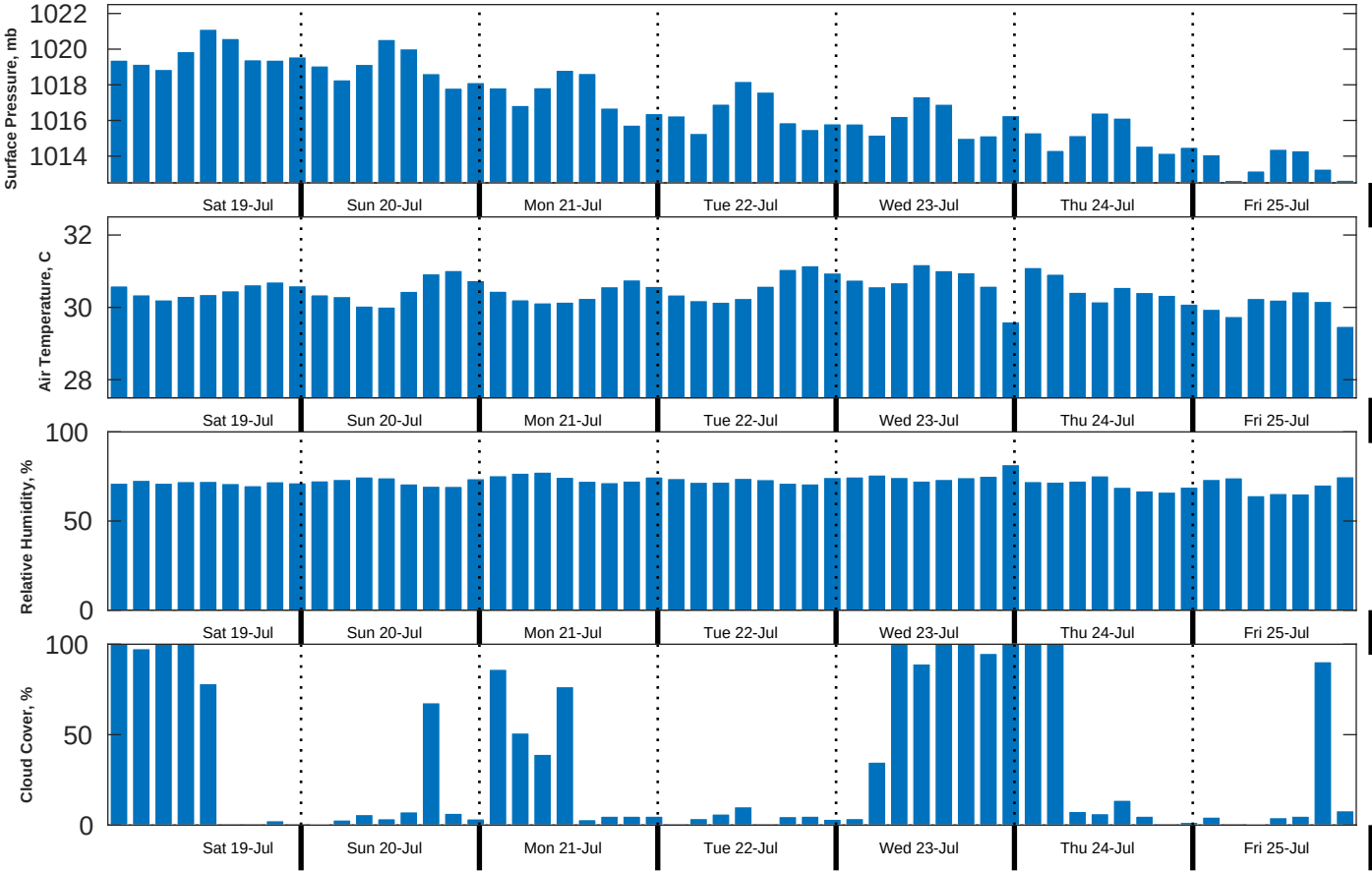
Met Forecast for Shell Noches GC19 PPL Geotechnical from 19-Jul-2025 00:00:00 to 26-Jul-2025 00:00:00
