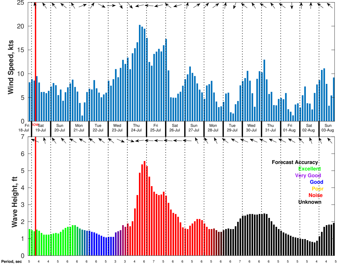
Wind & Wave Forecast for Shell Noches GC19 PPL Geotechnical from 18-Jul-2025 20:00:00 to 03-Aug-2025 20:00:00
