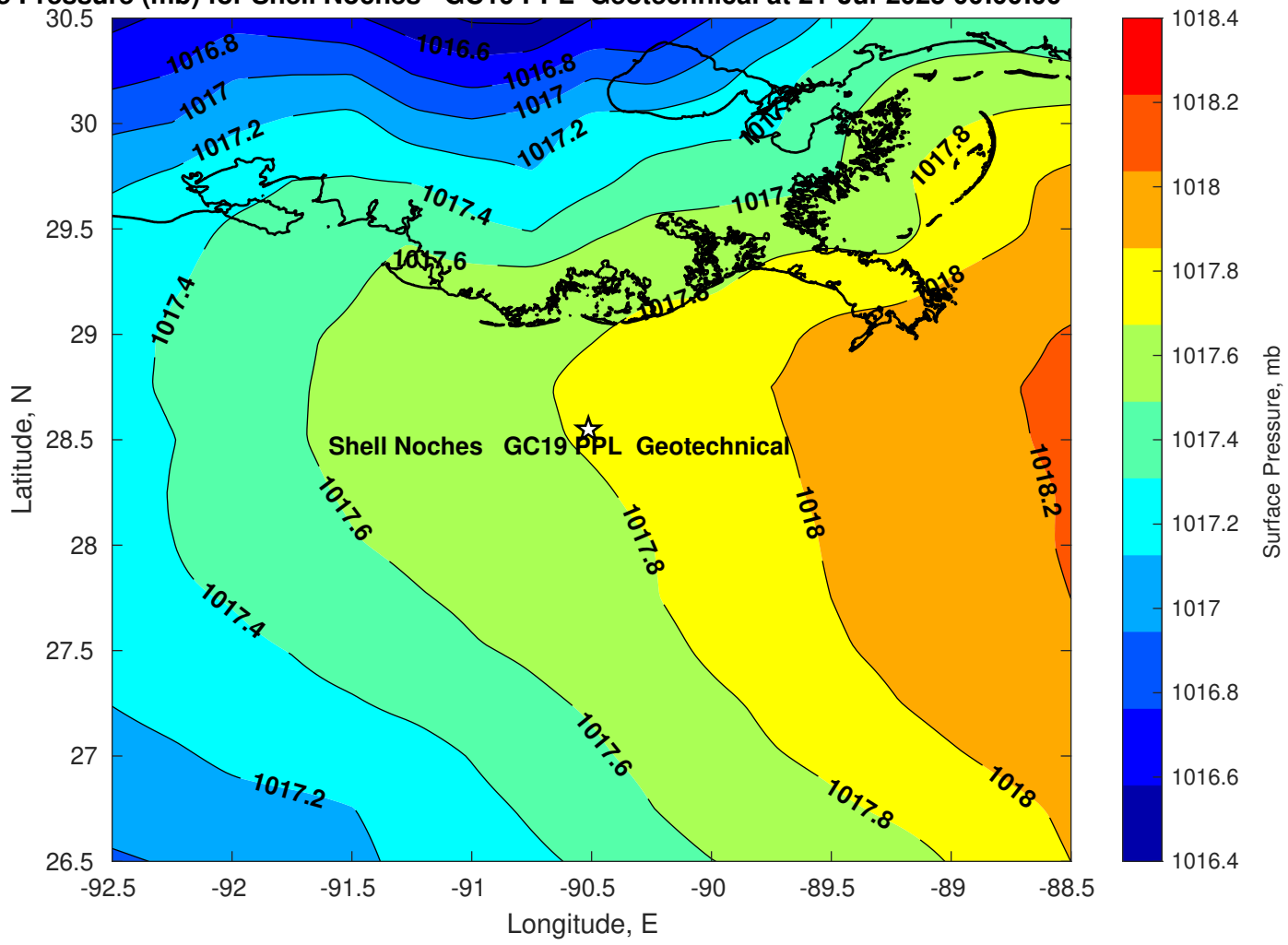
Surface Pressure (mb) for Shell Noches GC19 PPL Geotechnical at 21-Jul-2025 00:00:00
