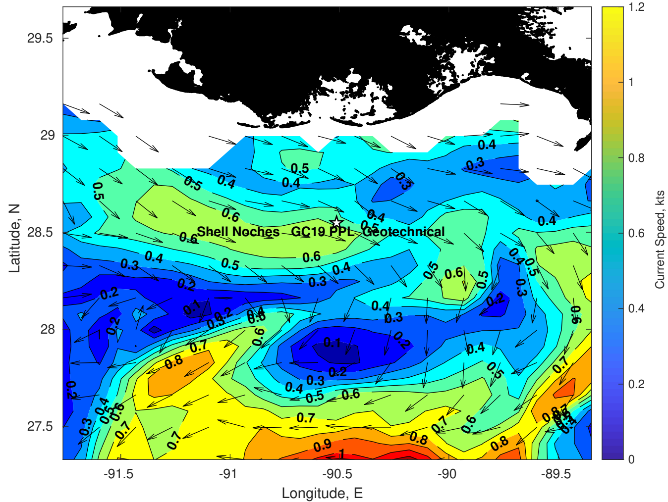
Surface Currents for Shell Noches GC19 PPL Geotechnical at 18-Jul-2025 00:00:00
