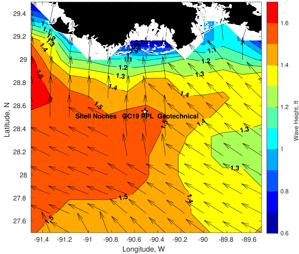
Wave Height (ft) for Shell Noches GC19 PPL Geotechnical at 19-Jul-2025 09:00:00
