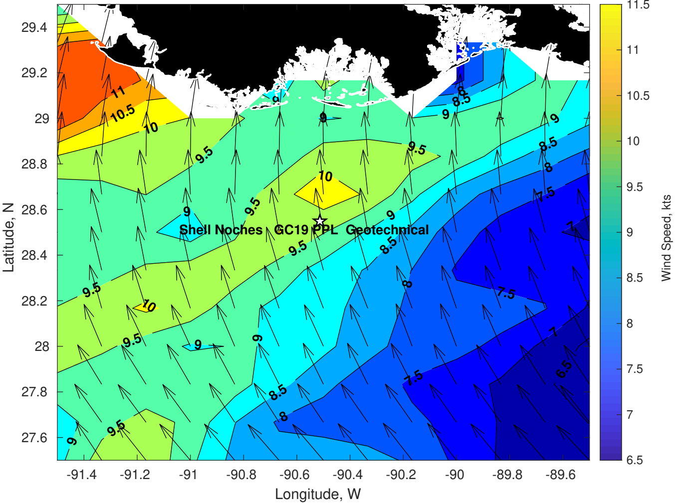
Winds (kts) for Shell Noches GC19 PPL Geotechnical at 19-Jul-2025 09:00:00
