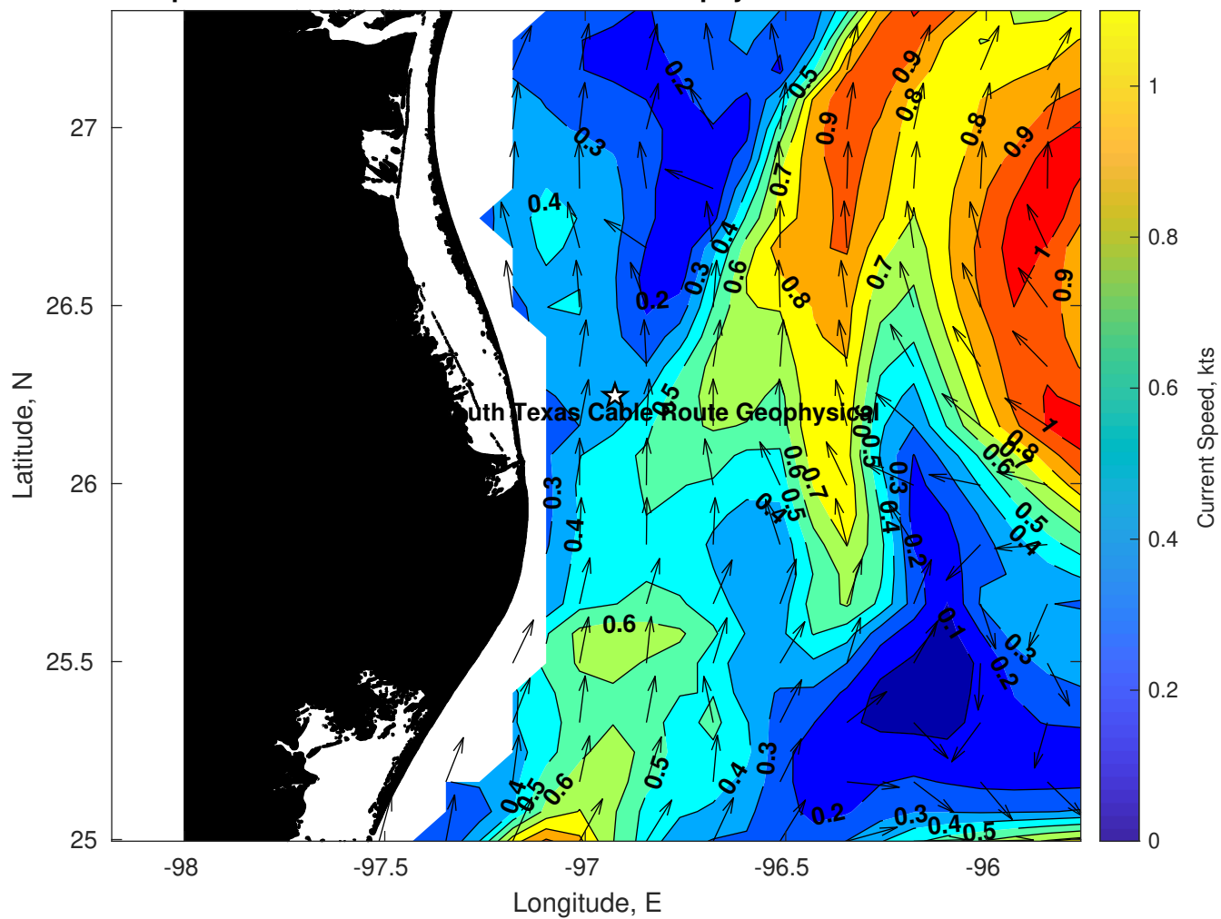
Surface Currents for Tampnet P2378 South Texas Cable Route Geophysical at 18-Jul-2025 00:00:00
