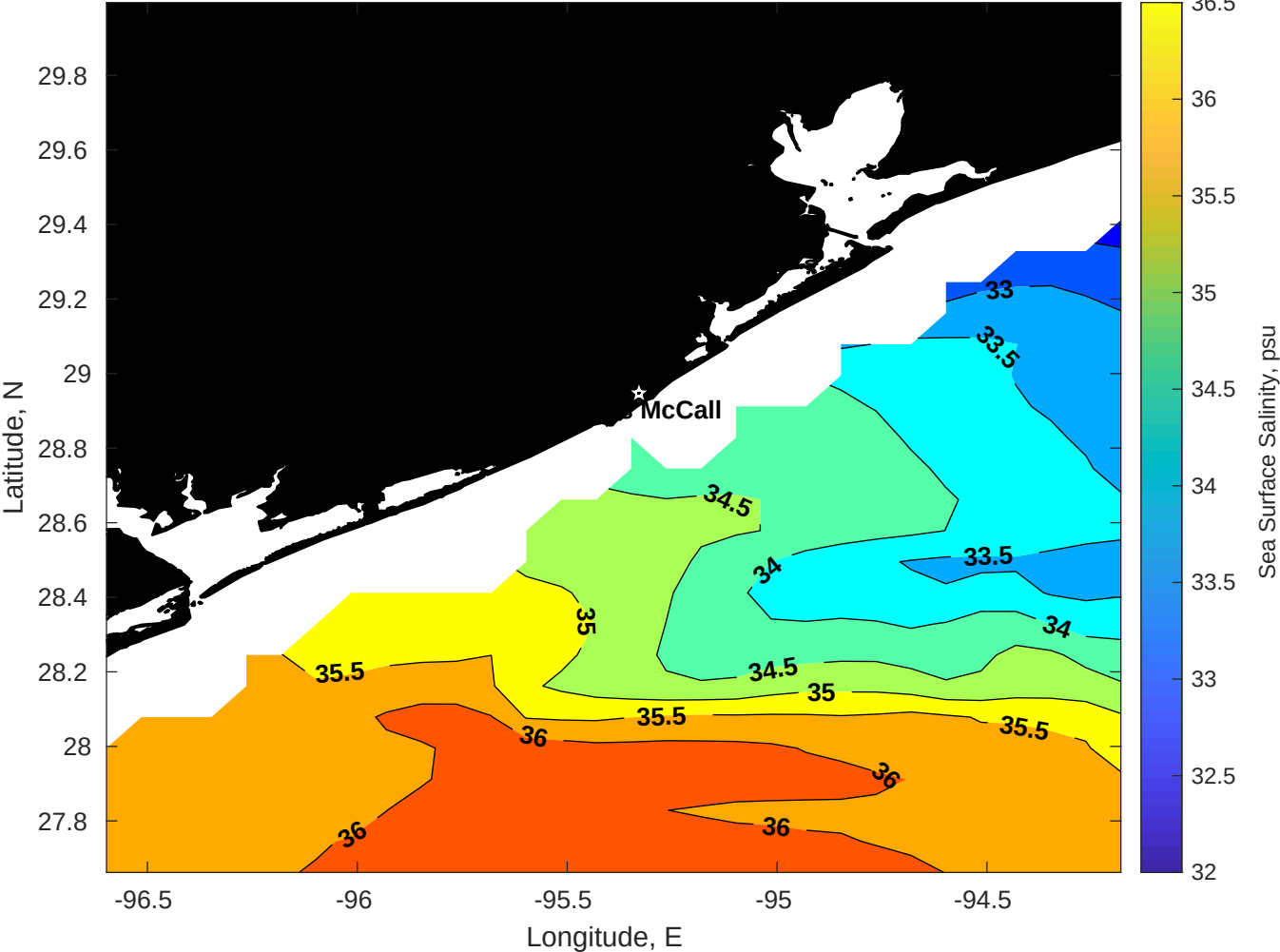
Surface Salinity for Brooks McCall at 19-Jul-2025 00:00:00
