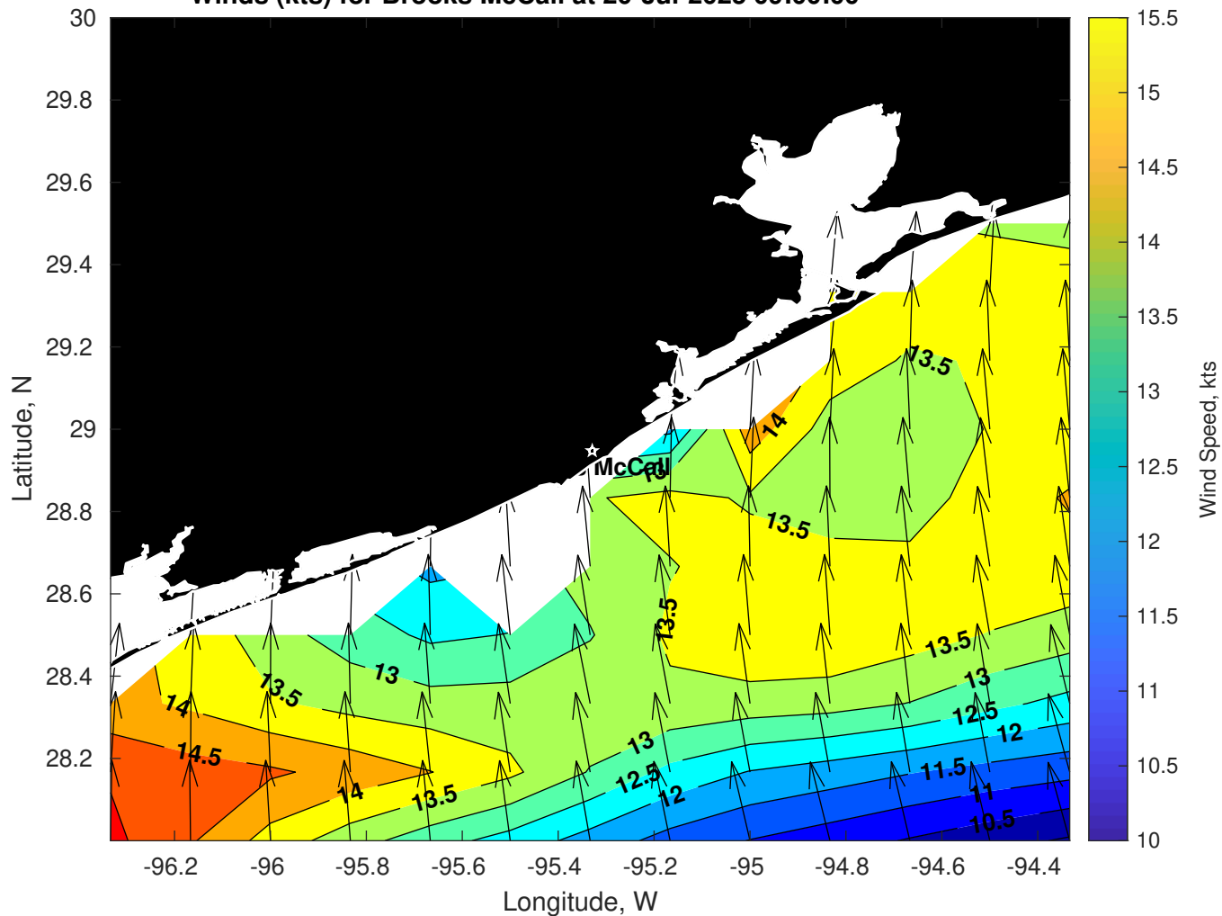
Winds (kts) for Brooks McCall at 20-Jul-2025 09:00:00
