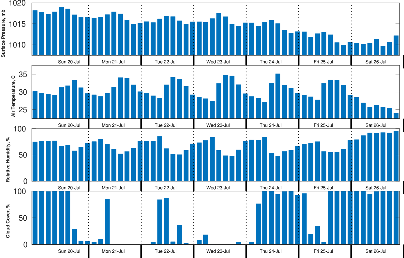
Met Forecast for Brooks McCall from 20-Jul-2025 00:00:00 to 27-Jul-2025 00:00:00
