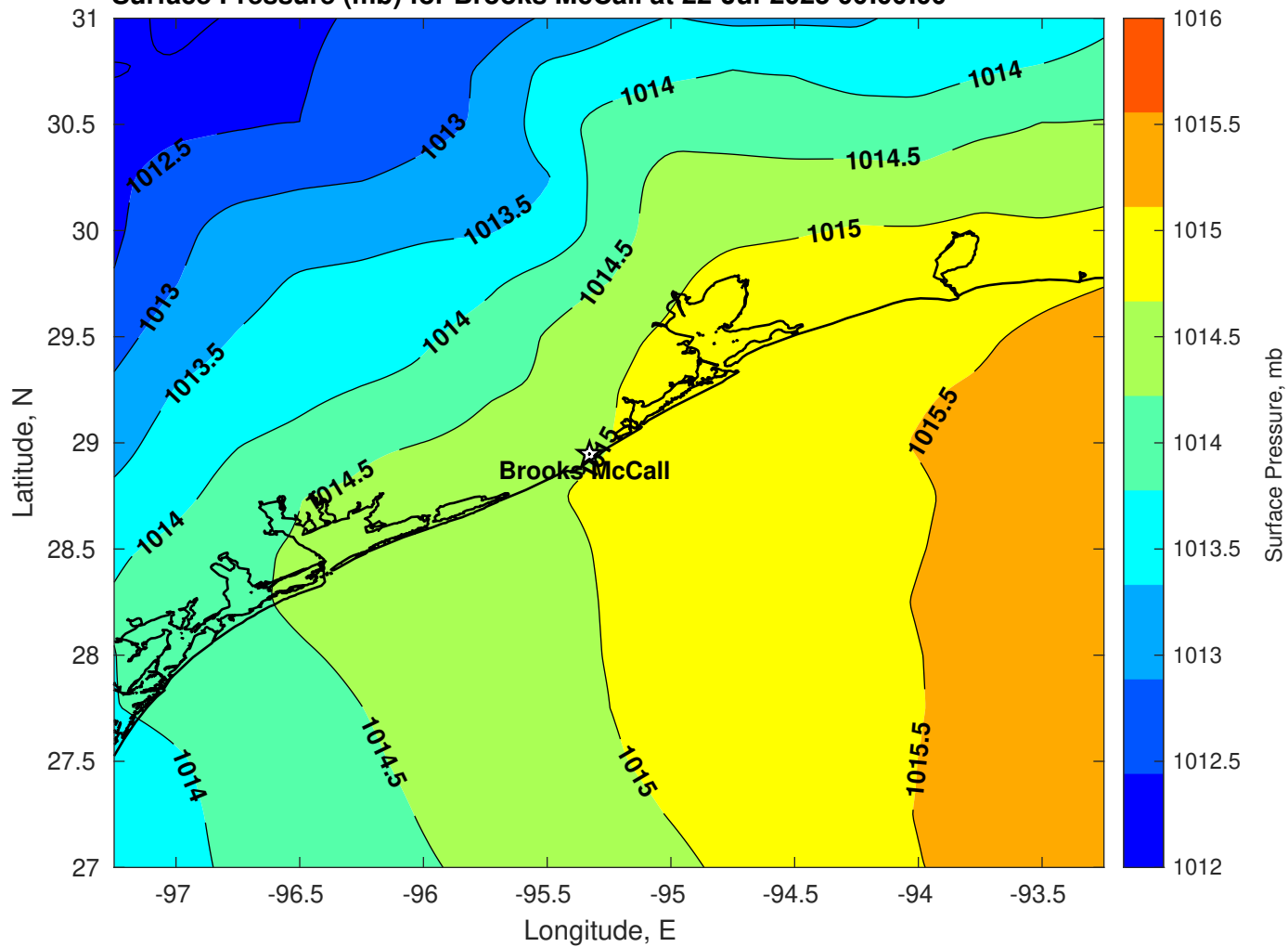
Surface Pressure (mb) for Brooks McCall at 22-Jul-2025 00:00:00
