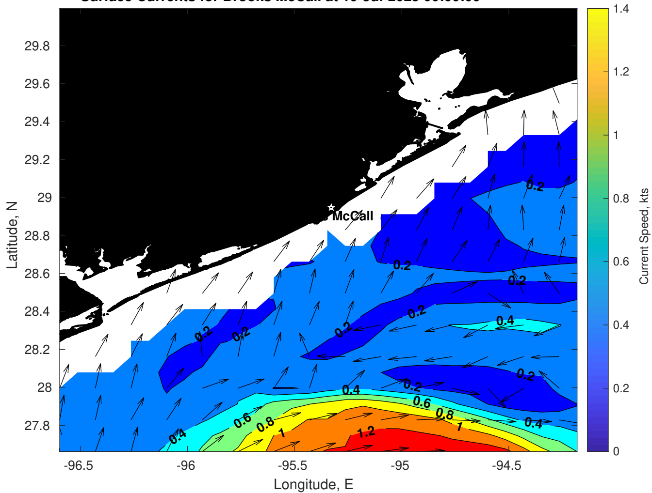
Surface Currents for Brooks McCall at 19-Jul-2025 00:00:00
