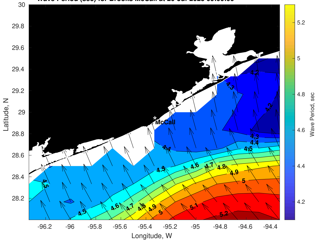
Wave Period (sec) for Brooks McCall at 20-Jul-2025 09:00:00
