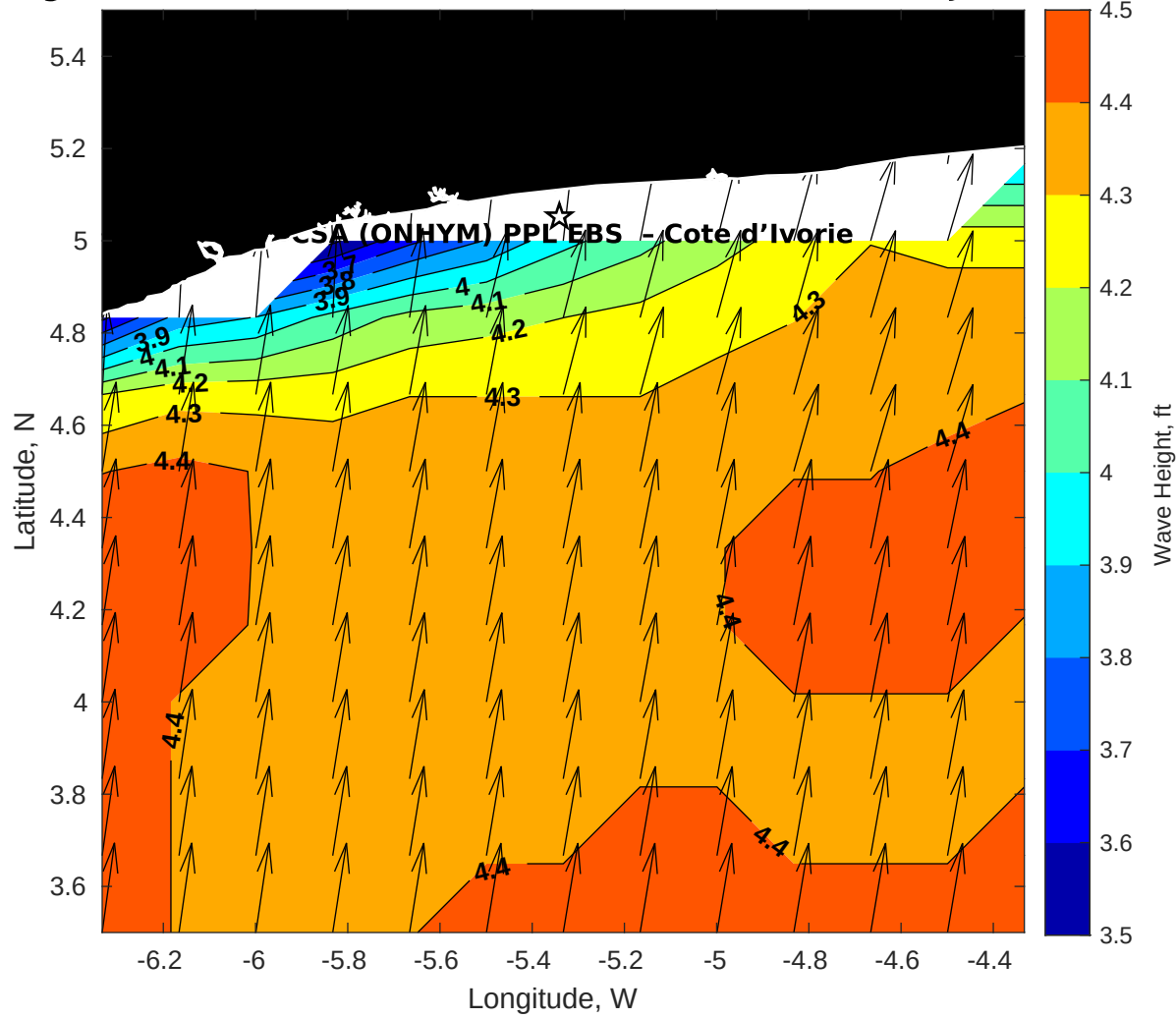
Wave Height (ft) for CSA (ONHYM) PPL EBS - Cote d'Ivoire at 19-Jul-2025 21:00:00
