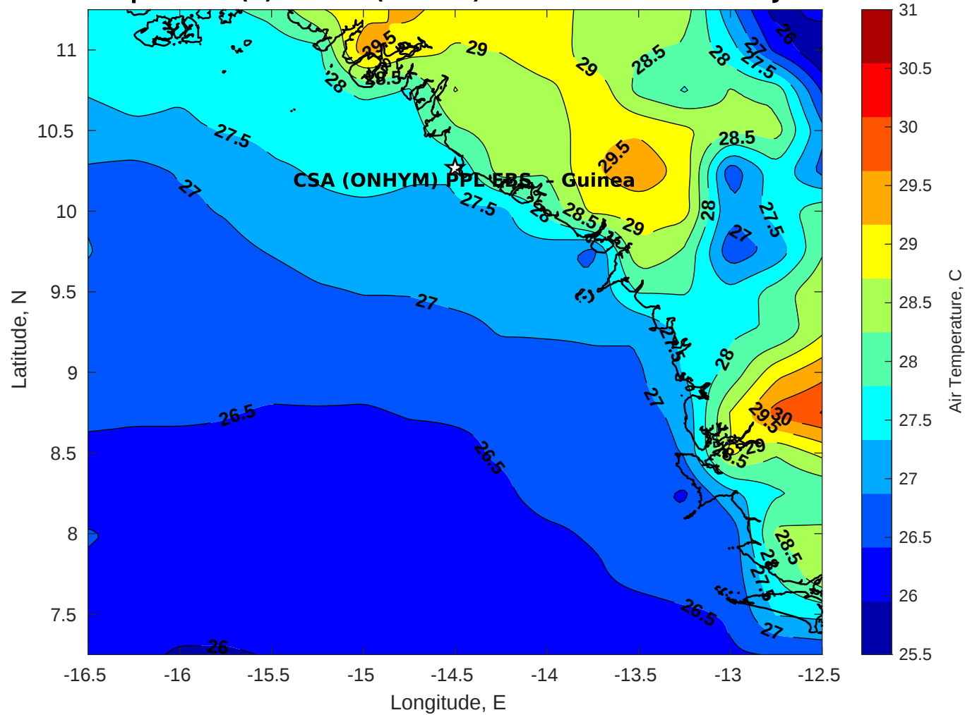
Air Temperature (C) for CSA (ONHYM) PPL EBS - Guinea at 19-Jul-2025
